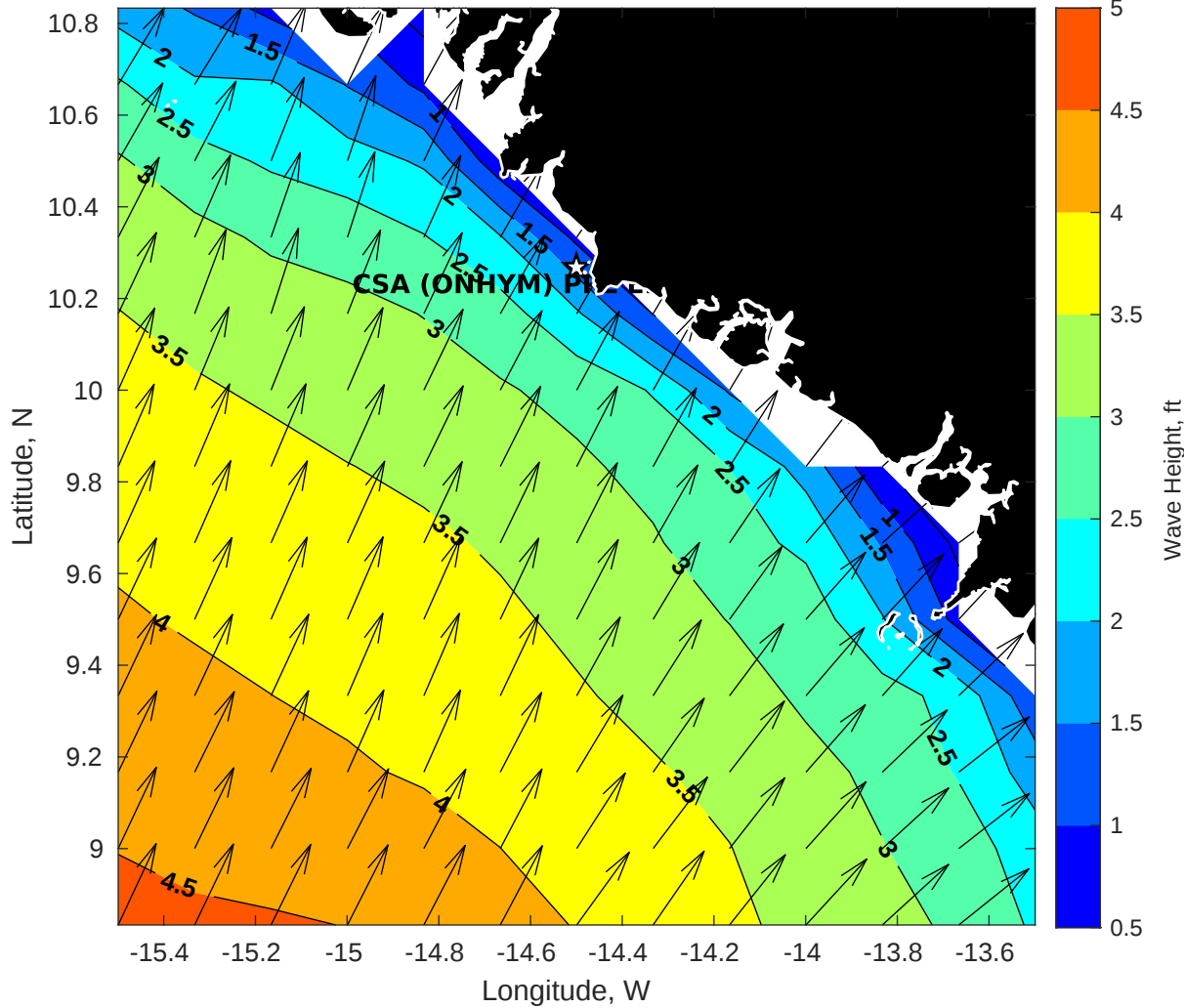
Wave Height (ft) for CSA (ONHYM) PPL EBS - Guinea at 01-Oct-2025 09:00:00
