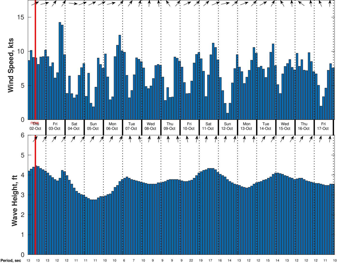
Wind & Wave Forecast for CSA (ONHYM) PPL EBS - Liberia from 01-Oct-2025 01:00:00 to 17-Oct-2025 01:00:00
