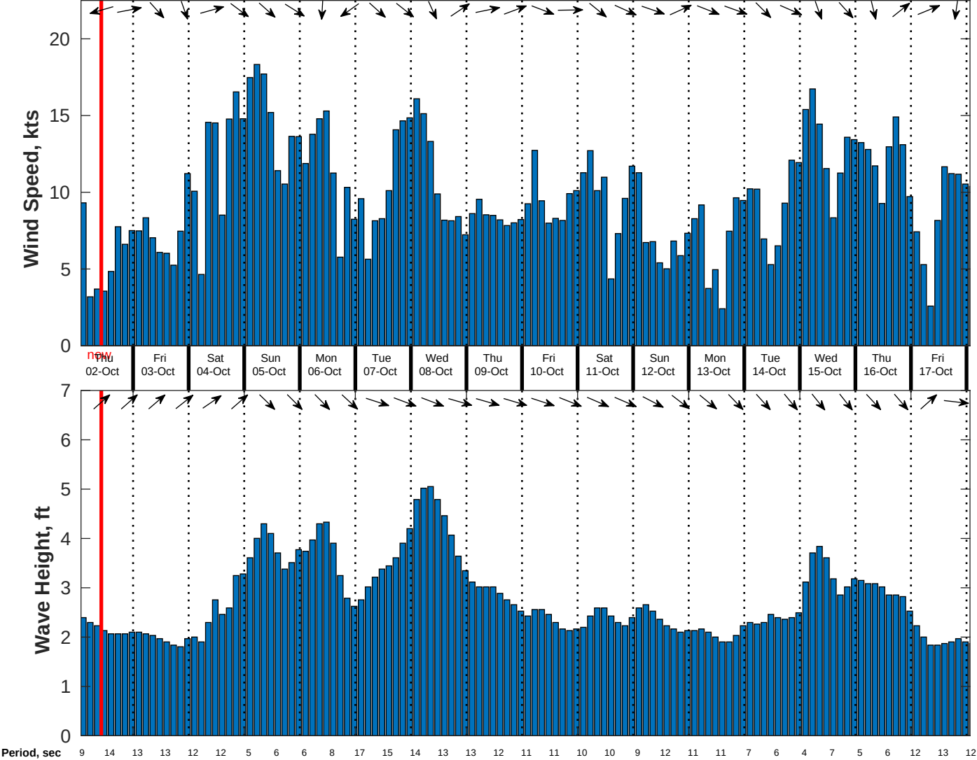
Wind & Wave Forecast for CSA (ONHYM) PPL EBS - Mauritania from 01-Oct-2025 01:00:00 to 17-Oct-2025 01:00:00
