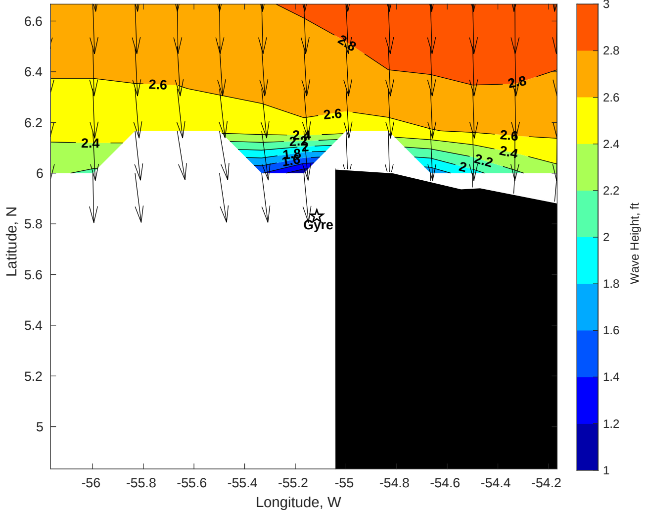
Wave Height (ft) for Gyre at 01-Oct-2025 09:00:00
