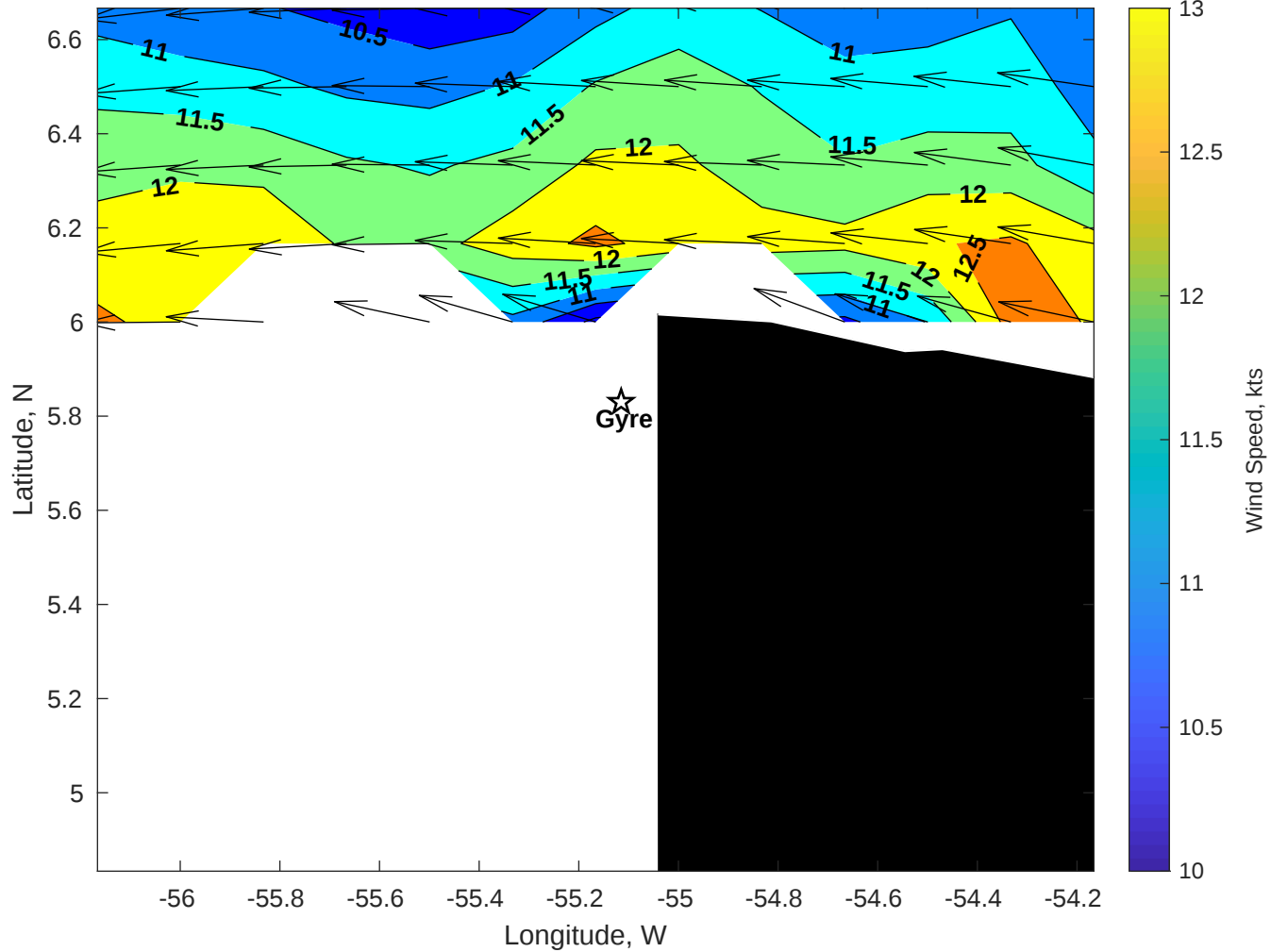
Winds (kts) for Gyre at 01-Oct-2025 09:00:00
