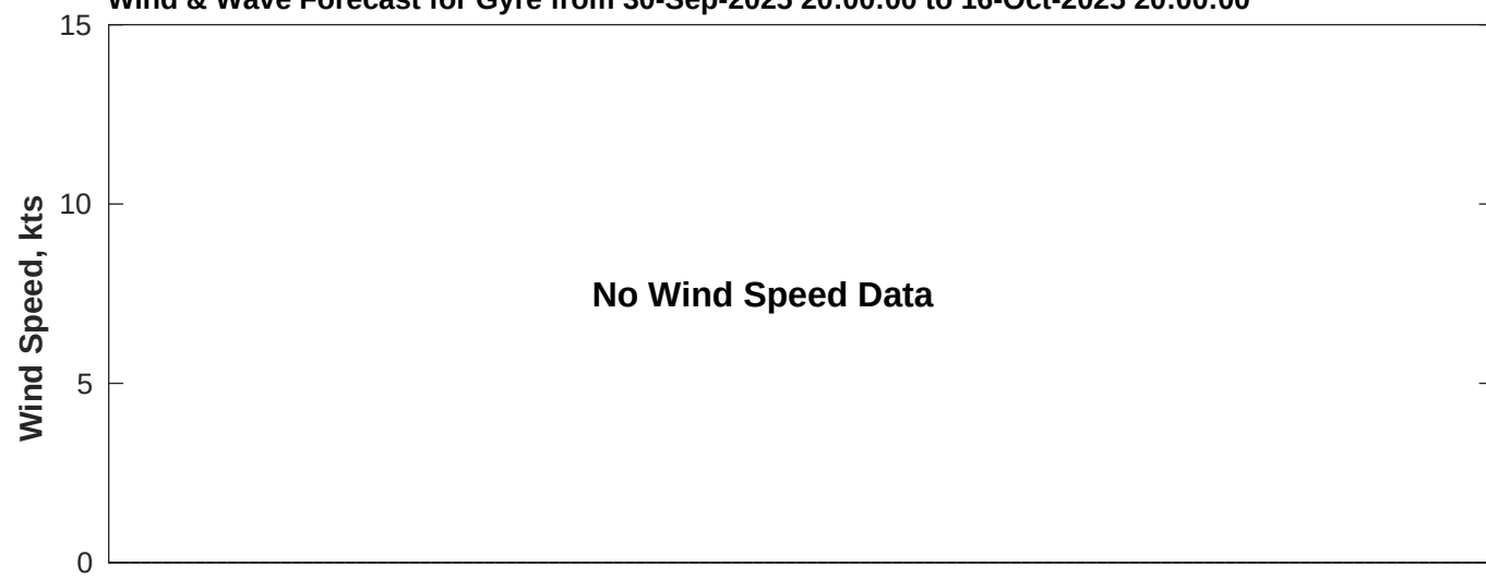
Wind & Wave Forecast for Gyre from 30-Sep-2025 20:00:00 to 16-Oct-2025 20:00:00
