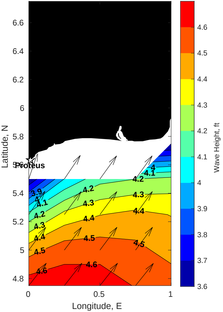
Wave Height (ft) for Proteus at 01-Oct-2025 09:00:00
