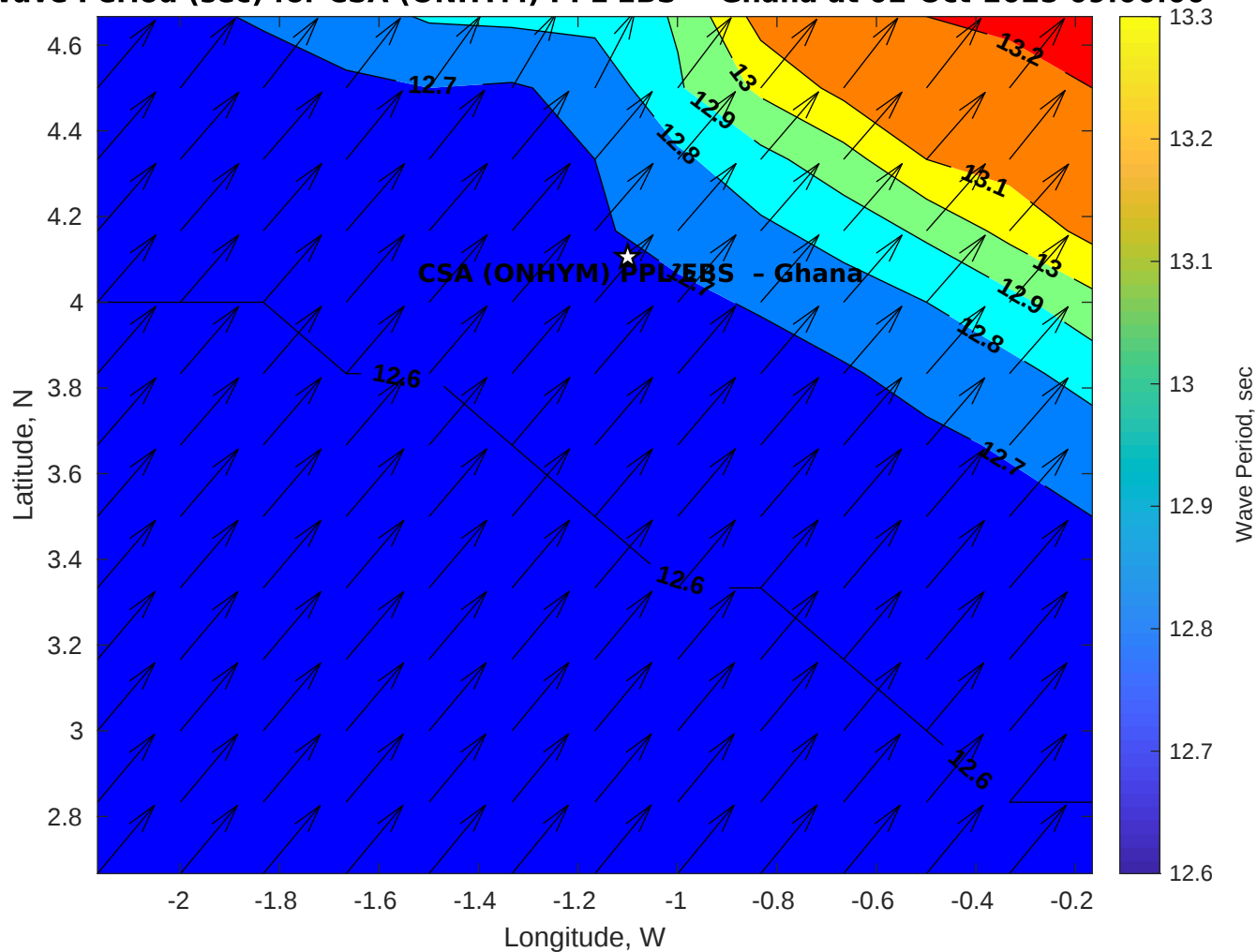
Wave Period (sec) for CSA (ONHYM) PPL EBS - Ghana at 02-Oct-2025 09:00:00
