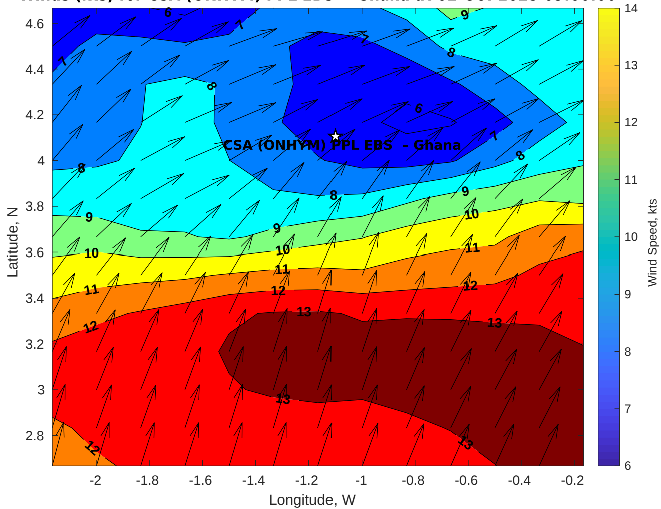
Winds (kts) for CSA (ONHYM) PPL EBS - Ghana at 02-Oct-2025 09:00:00
