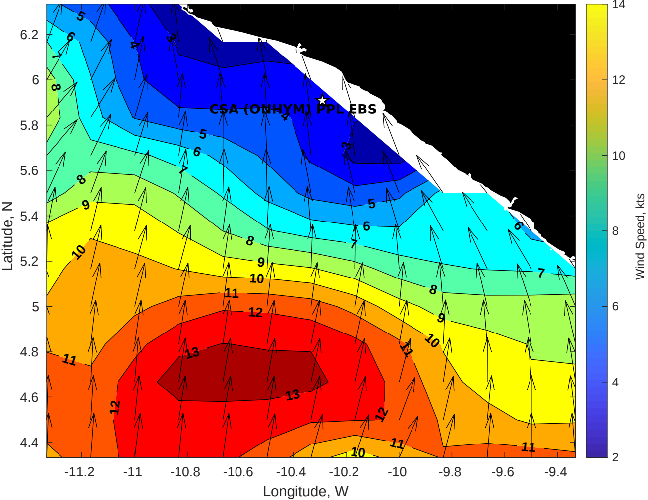
Winds (kts) for CSA (ONHYM) PPL EBS - Liberia at 02-Oct-2025 09:00:00
