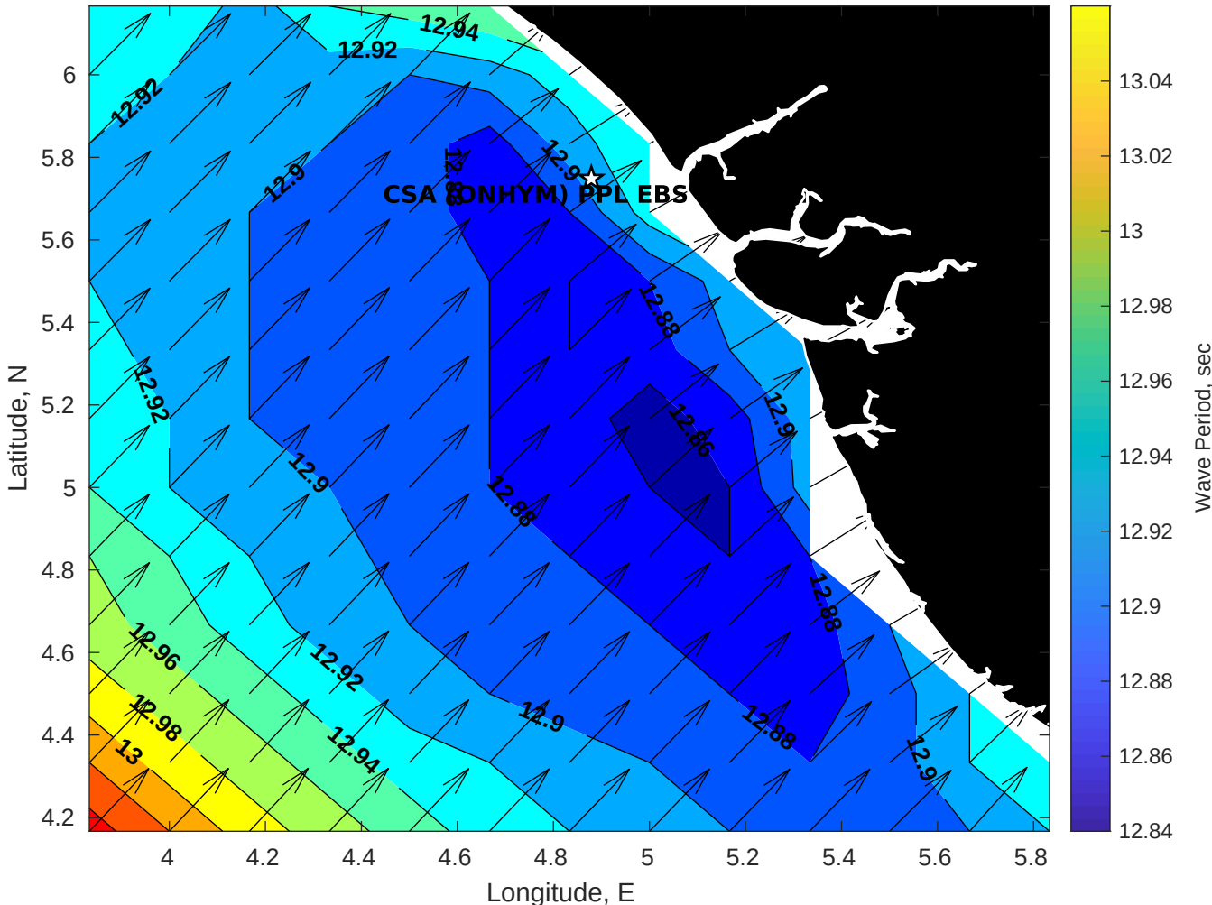
Wave Period (sec) for CSA (ONHYM) PPL EBS - Nigeria at 02-Oct-2025 09:00:00
