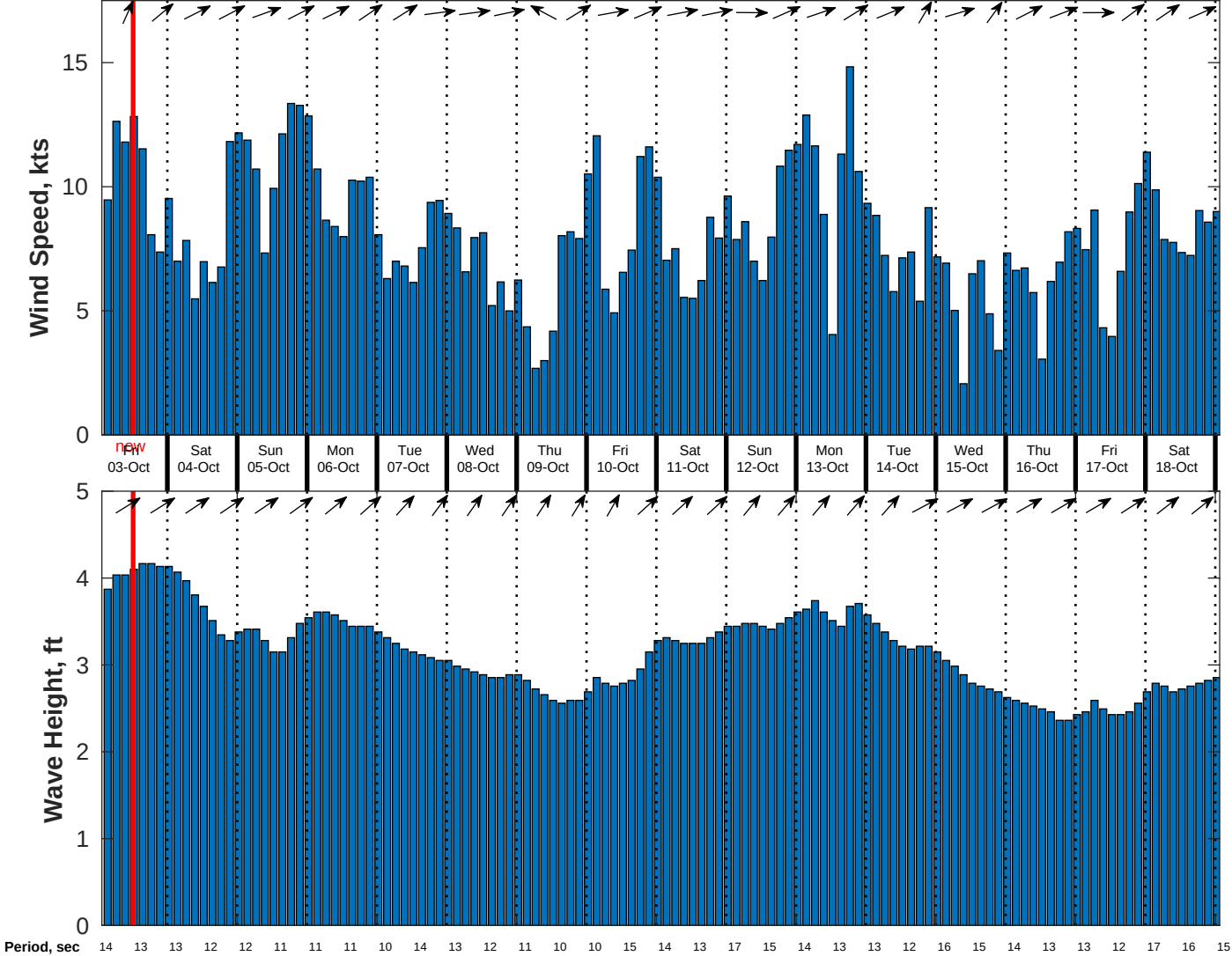
Wind & Wave Forecast for CSA (ONHYM) PPL EBS - Nigeria from 02-Oct-2025 02:00:00 to 18-Oct-2025 02:00:00
