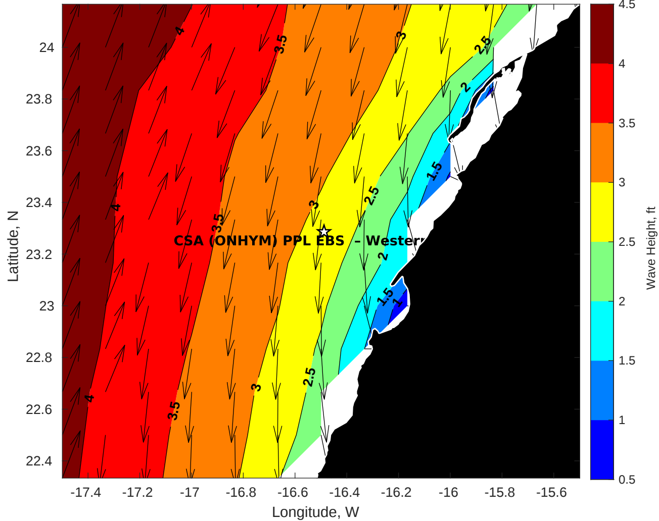
Wave Height (ft) for CSA (ONHYM) PPL EBS - Western Sahara at 02-Oct-2025 09:00:00
