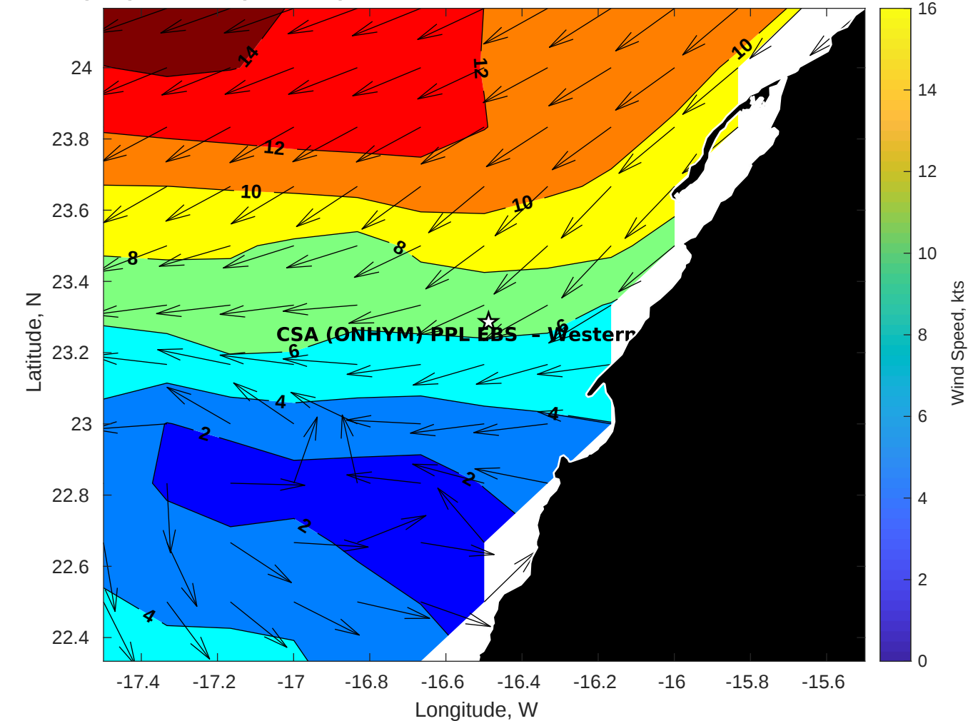
Winds (kts) for CSA (ONHYM) PPL EBS - Western Sahara at 02-Oct-2025 09:00:00
