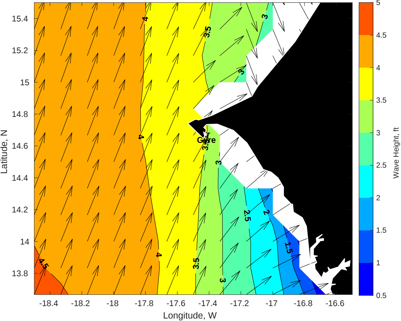
Wave Height (ft) for Gyre at 02-Oct-2025 09:00:00
