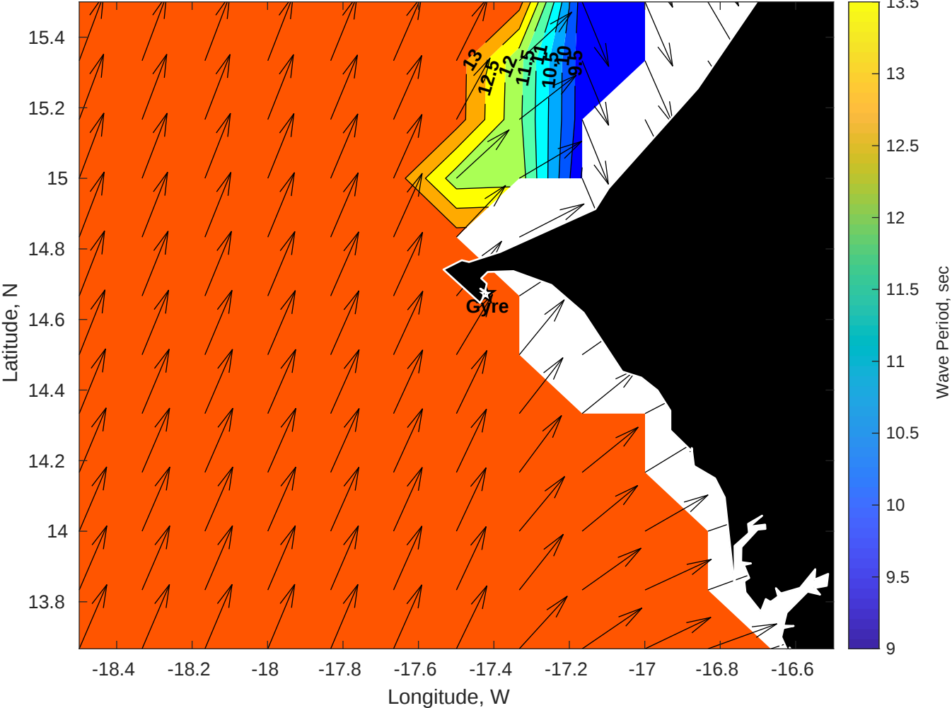
Wave Period (sec) for Gyre at 02-Oct-2025 09:00:00
