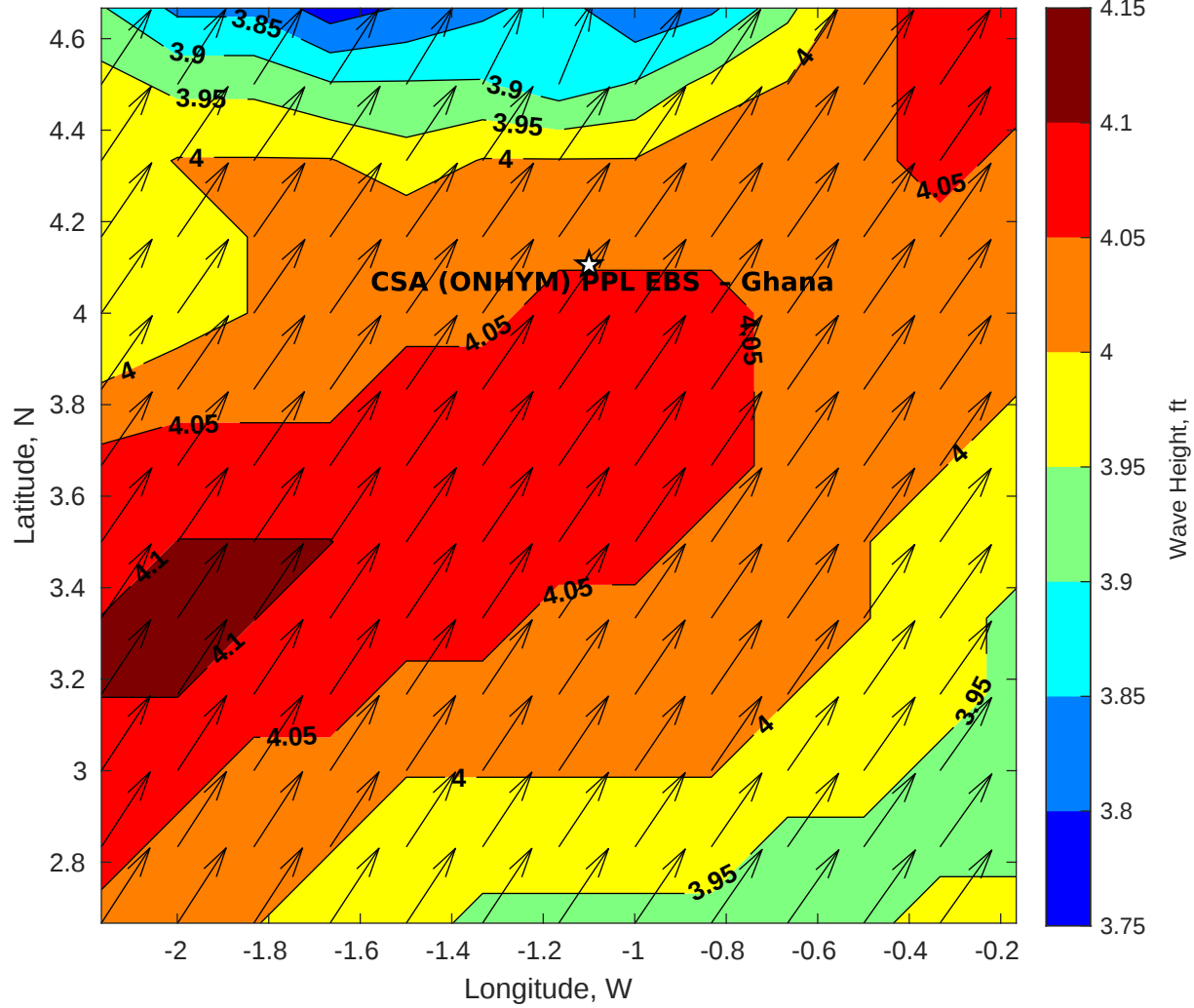
Wave Height (ft) for CSA (ONHYM) PPL EBS - Ghana at 03-Oct-2025 09:00:00
