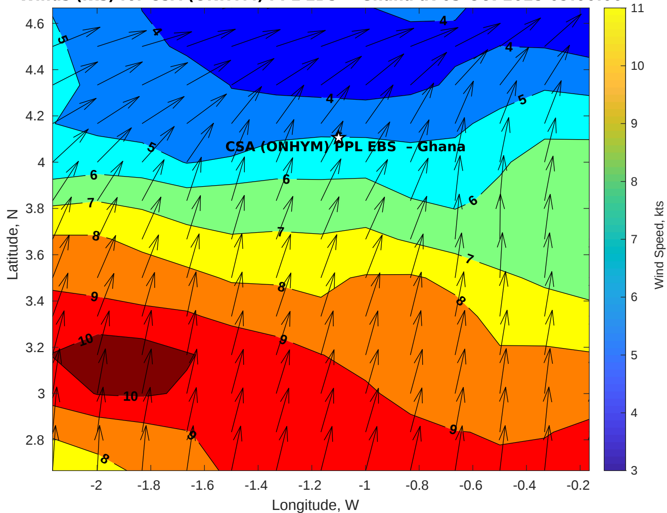
Winds (kts) for CSA (ONHYM) PPL EBS - Ghana at 03-Oct-2025 09:00:00
