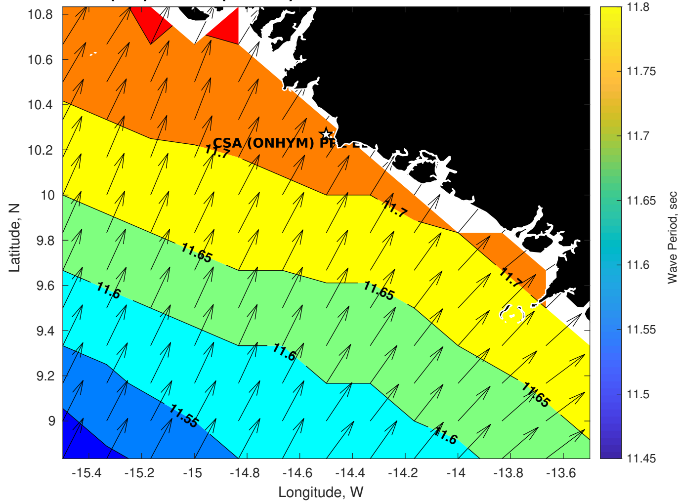
Wave Period (sec) for CSA (ONHYM) PPL EBS - Guinea at 03-Oct-2025 09:00:00
