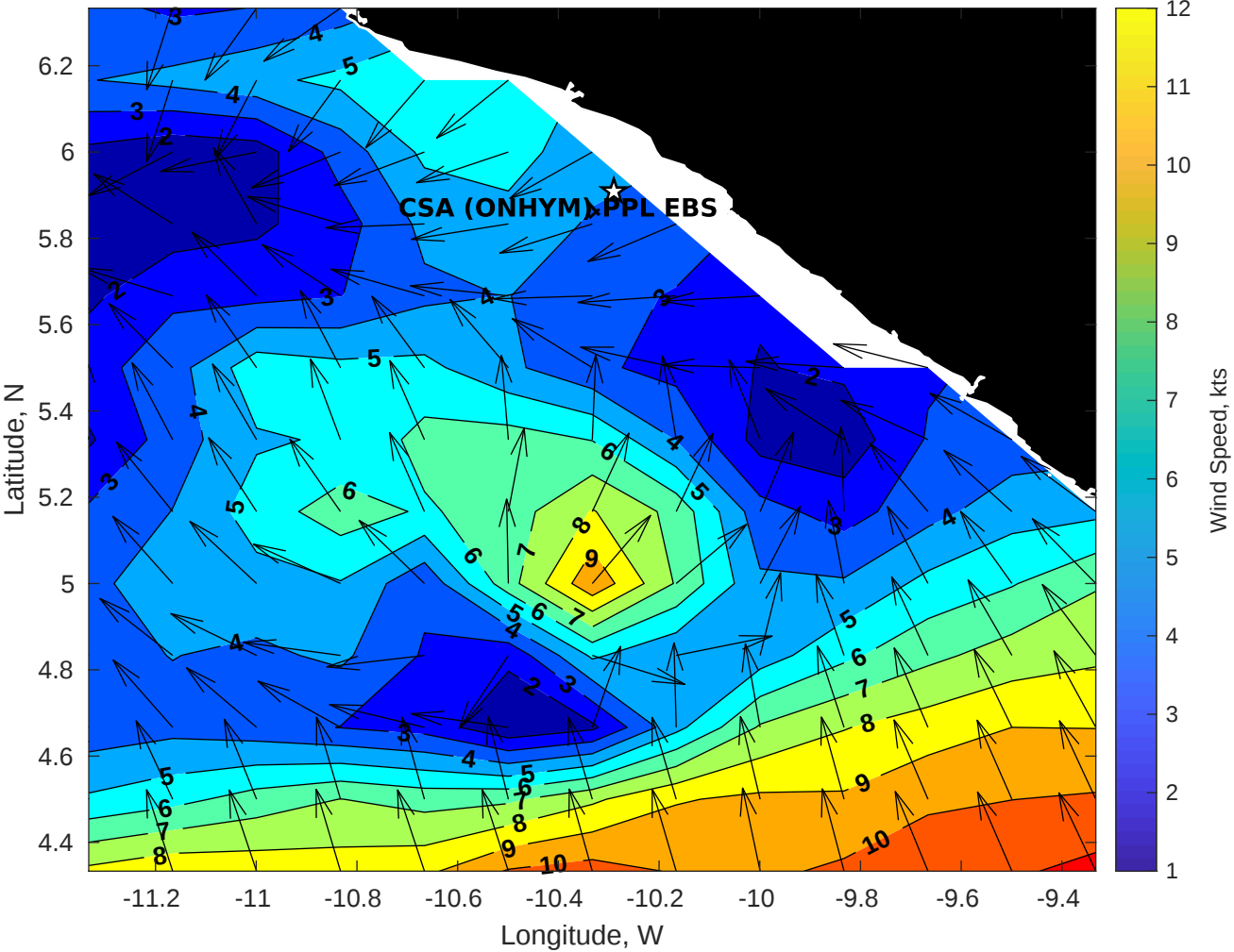
Winds (kts) for CSA (ONHYM) PPL EBS - Liberia at 03-Oct-2025 09:00:00
