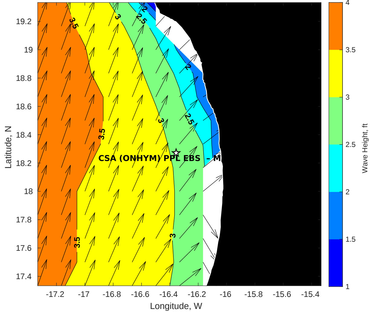
Wave Height (ft) for CSA (ONHYM) PPL EBS - Mauritania at 03-Oct-2025 09:00:00
