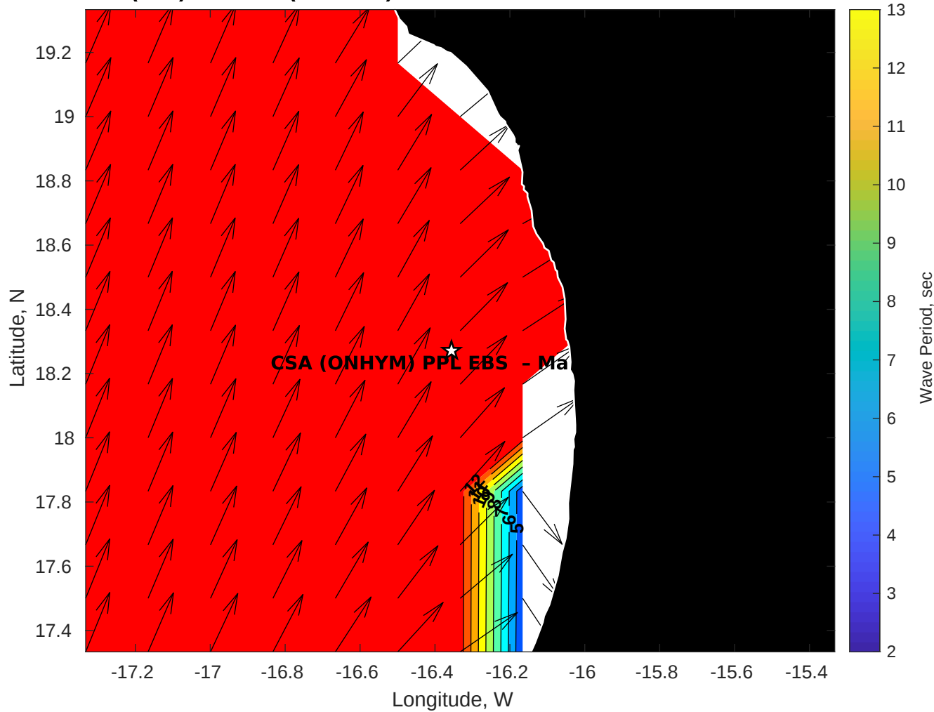
Wave Period (sec) for CSA (ONHYM) PPL EBS - Mauritania at 03-Oct-2025 09:00:00
