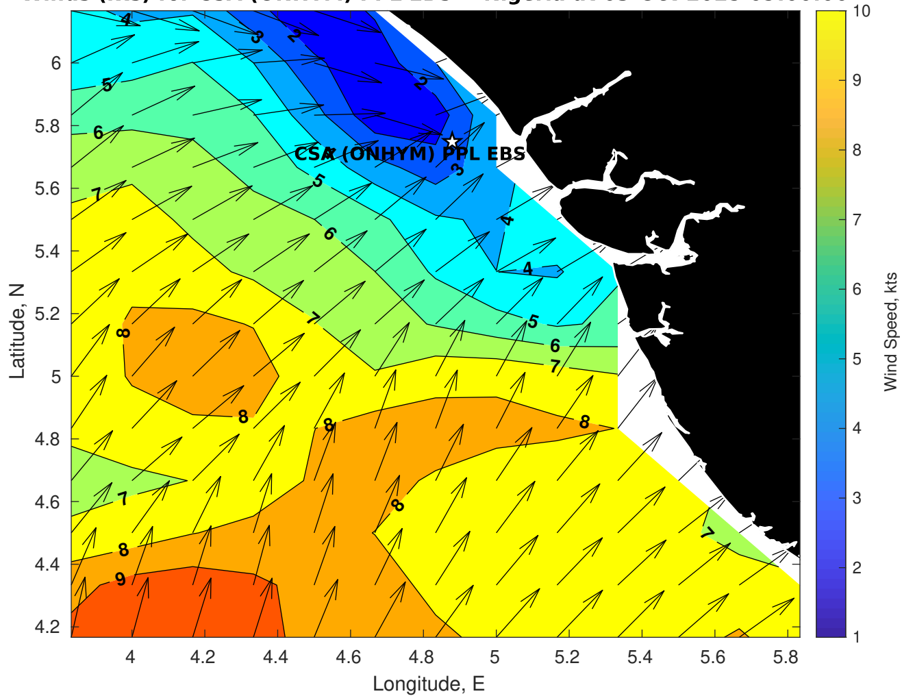
Winds (kts) for CSA (ONHYM) PPL EBS - Nigeria at 03-Oct-2025 09:00:00
