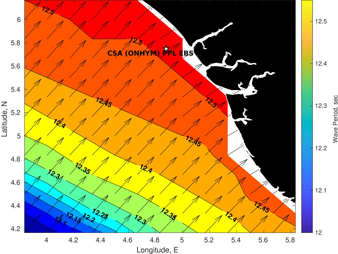
Wave Period (sec) for CSA (ONHYM) PPL EBS - Nigeria at 03-Oct-2025 09:00:00
