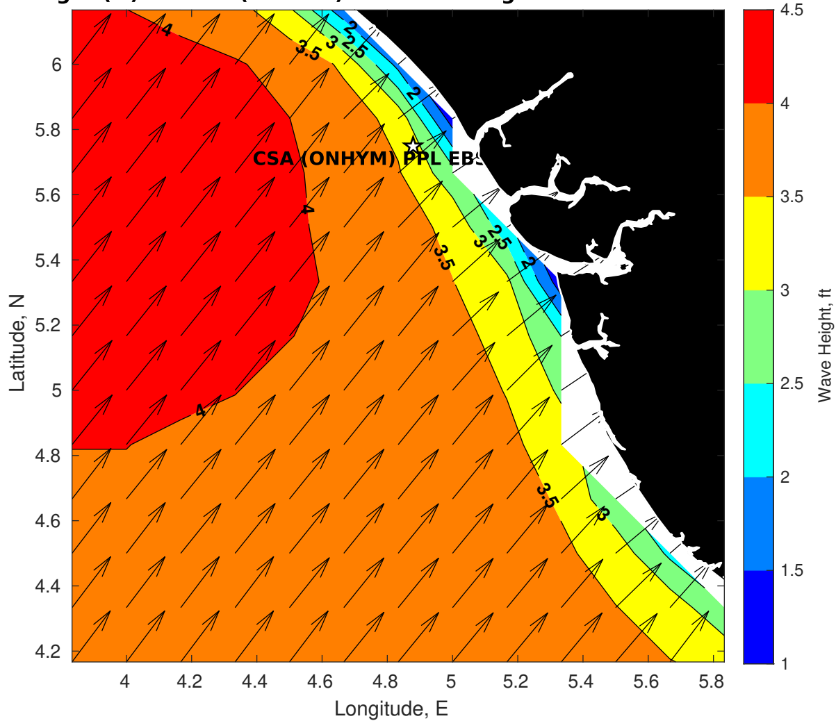
Wave Height (ft) for CSA (ONHYM) PPL EBS - Nigeria at 03-Oct-2025 09:00:00
