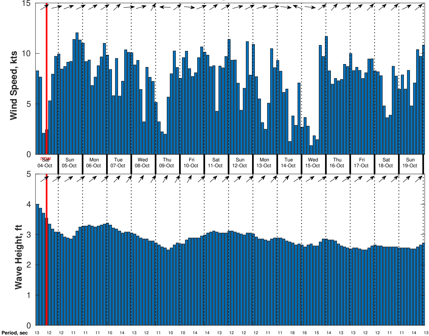
Wind & Wave Forecast for CSA (ONHYM) PPL EBS - Nigeria from 03-Oct-2025 02:00:00 to 19-Oct-2025 02:00:00
