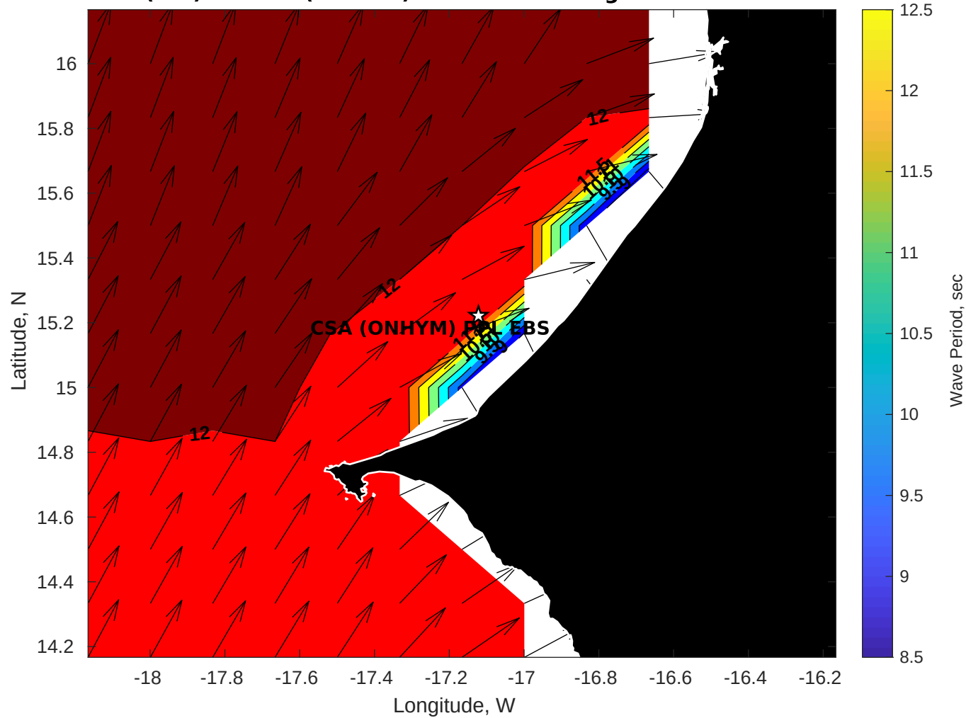
Wave Period (sec) for CSA (ONHYM) PPL EBS - Senegal at 03-Oct-2025 09:00:00
