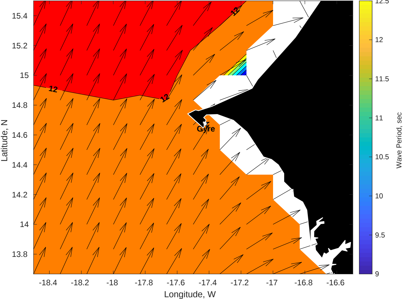
Wave Period (sec) for Gyre at 03-Oct-2025 09:00:00
