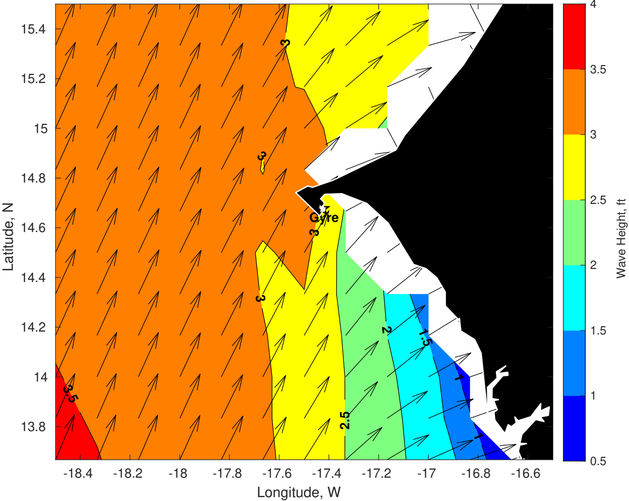
Wave Height (ft) for Gyre at 03-Oct-2025 09:00:00
