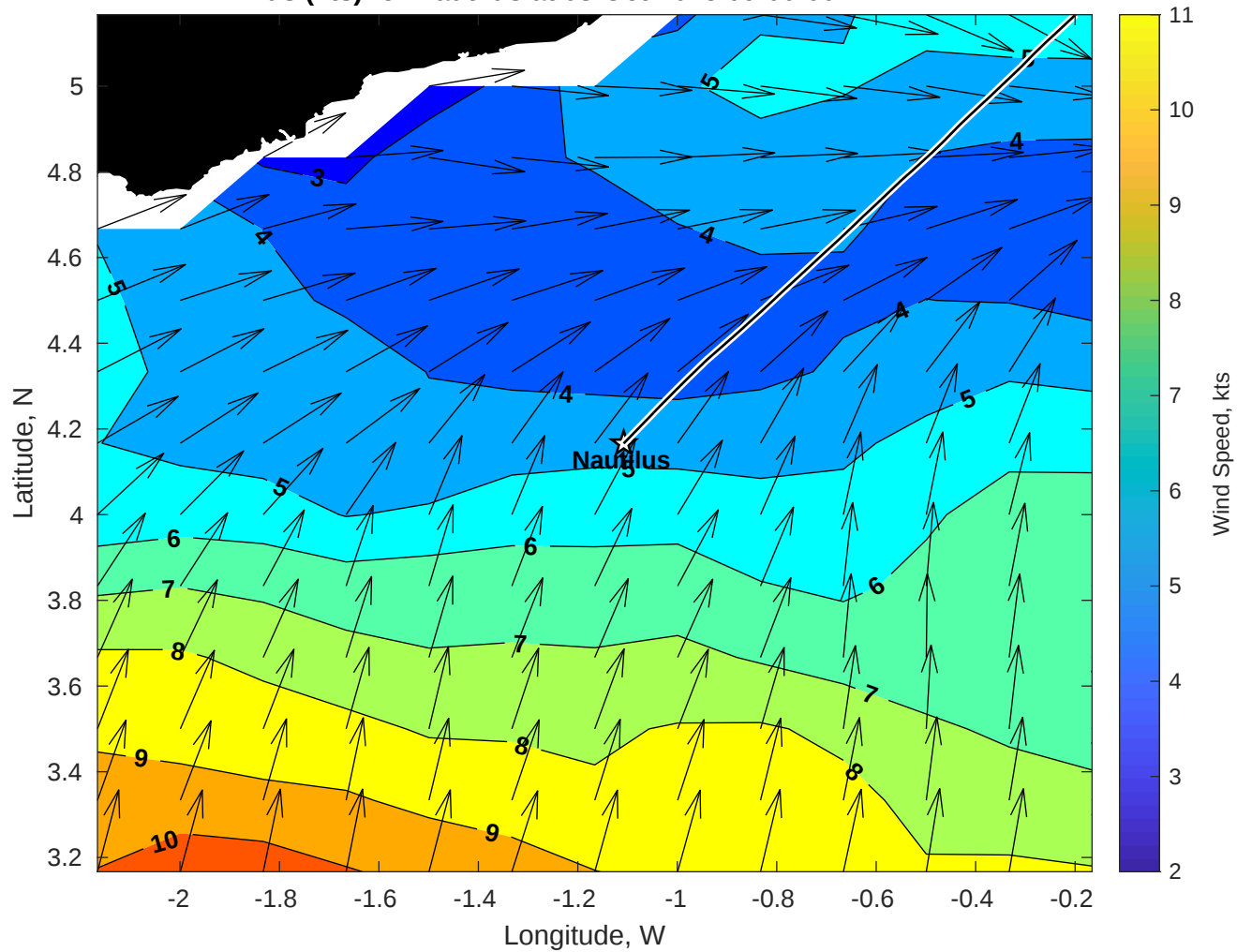
Winds (kts) for Nautilus at 03-Oct-2025 09:00:00
