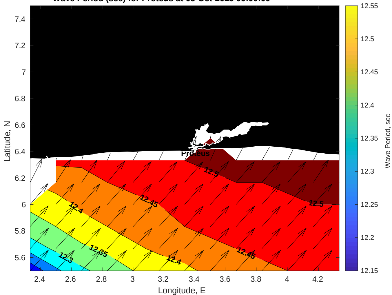
Wave Period (sec) for Proteus at 03-Oct-2025 09:00:00
