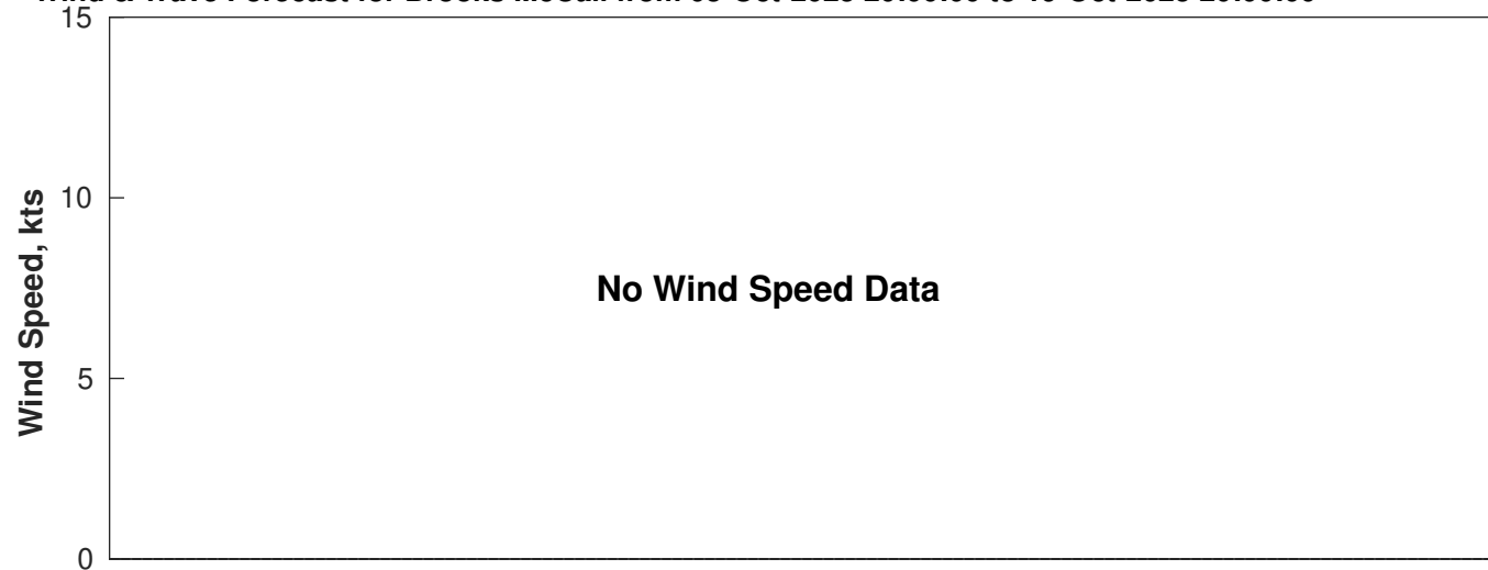
Wind & Wave Forecast for Brooks McCall from 03-Oct-2025 20:00:00 to 19-Oct-2025 20:00:00
