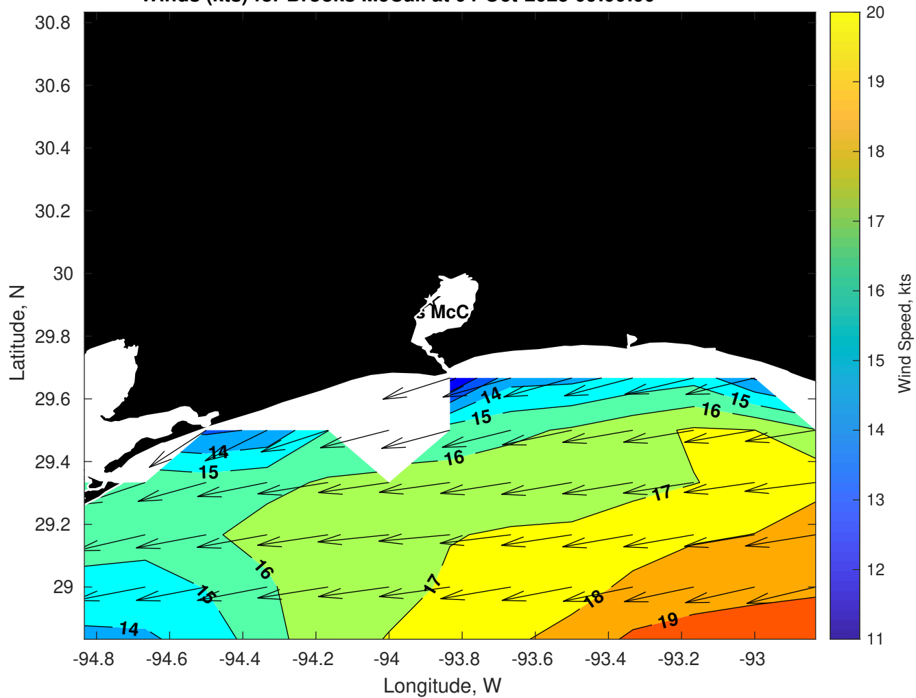
Winds (kts) for Brooks McCall at 04-Oct-2025 09:00:00
