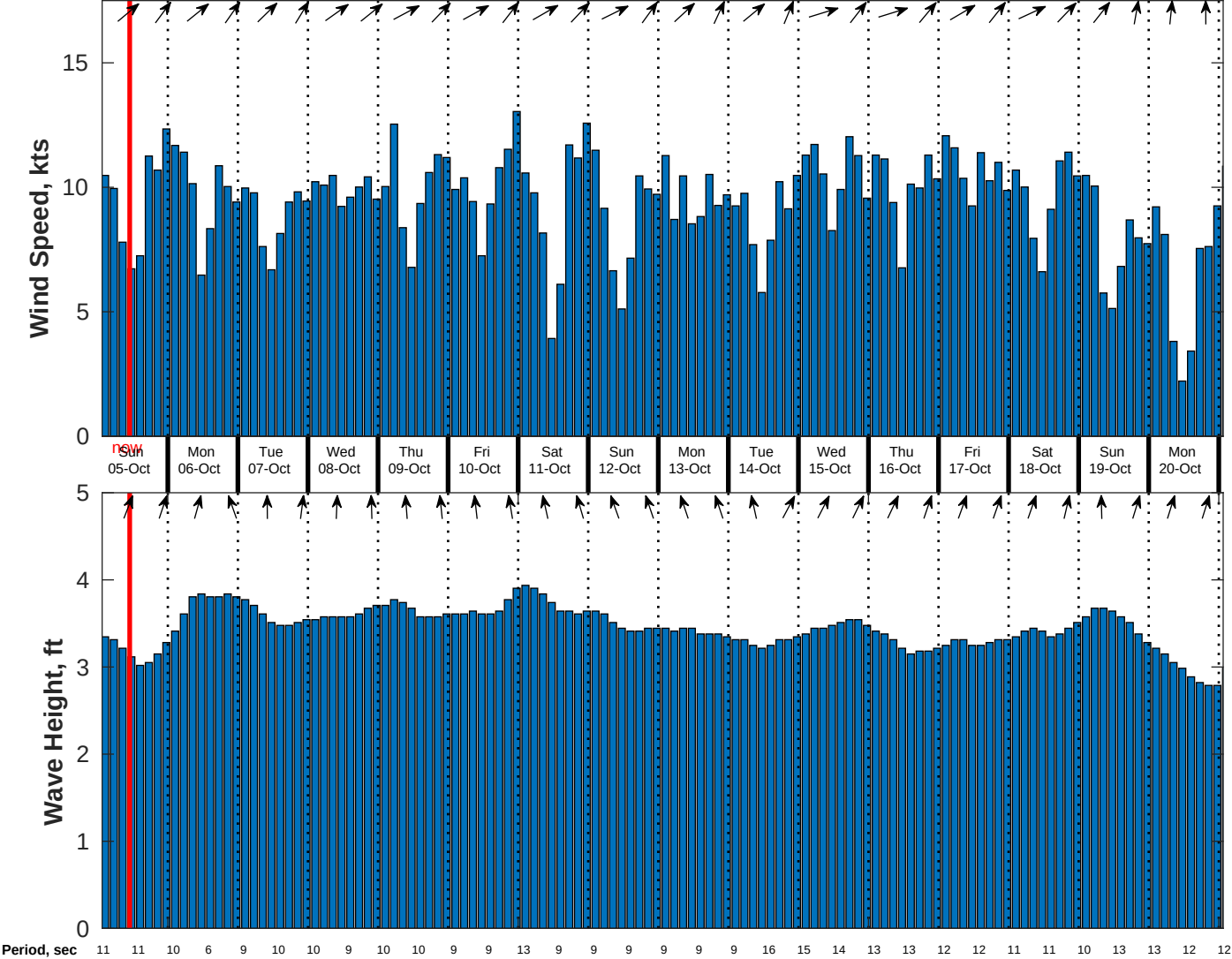
Wind & Wave Forecast for CSA (ONHYM) PPL EBS - Cote d'Ivoire from 04-Oct-2025 01:00:00 to 20-Oct-2025 01:00:00
