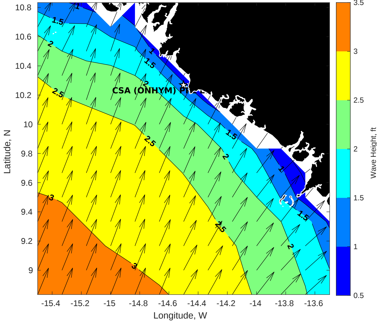
Wave Height (ft) for CSA (ONHYM) PPL EBS - Guinea at 04-Oct-2025 09:00:00
