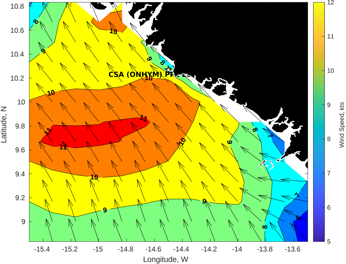
Winds (kts) for CSA (ONHYM) PPL EBS - Guinea at 04-Oct-2025 09:00:00
