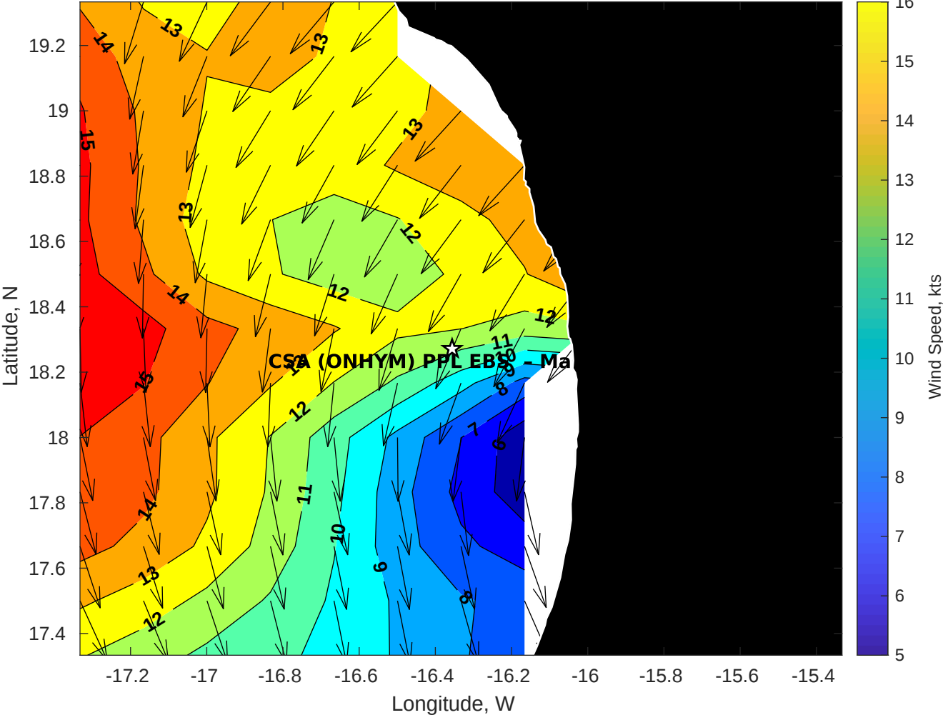
Winds (kts) for CSA (ONHYM) PPL EBS - Mauritania at 04-Oct-2025 09:00:00
