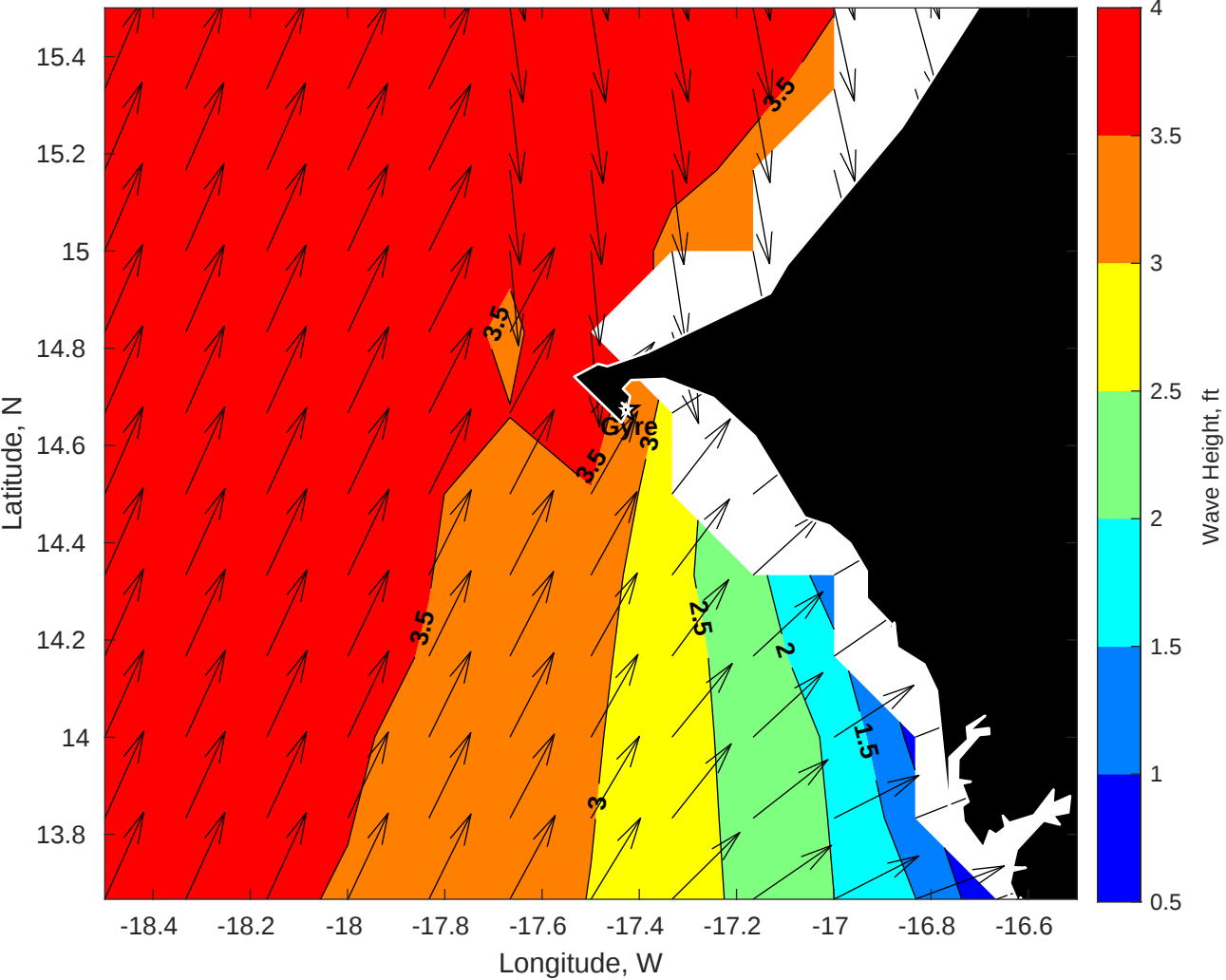
Wave Height (ft) for Gyre at 04-Oct-2025 09:00:00
