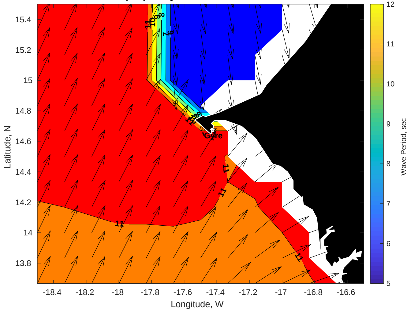
Wave Period (sec) for Gyre at 04-Oct-2025 09:00:00
