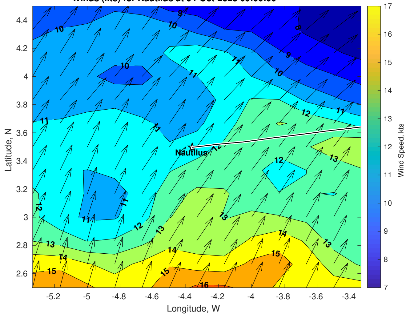
Winds (kts) for Nautilus at 04-Oct-2025 09:00:00
