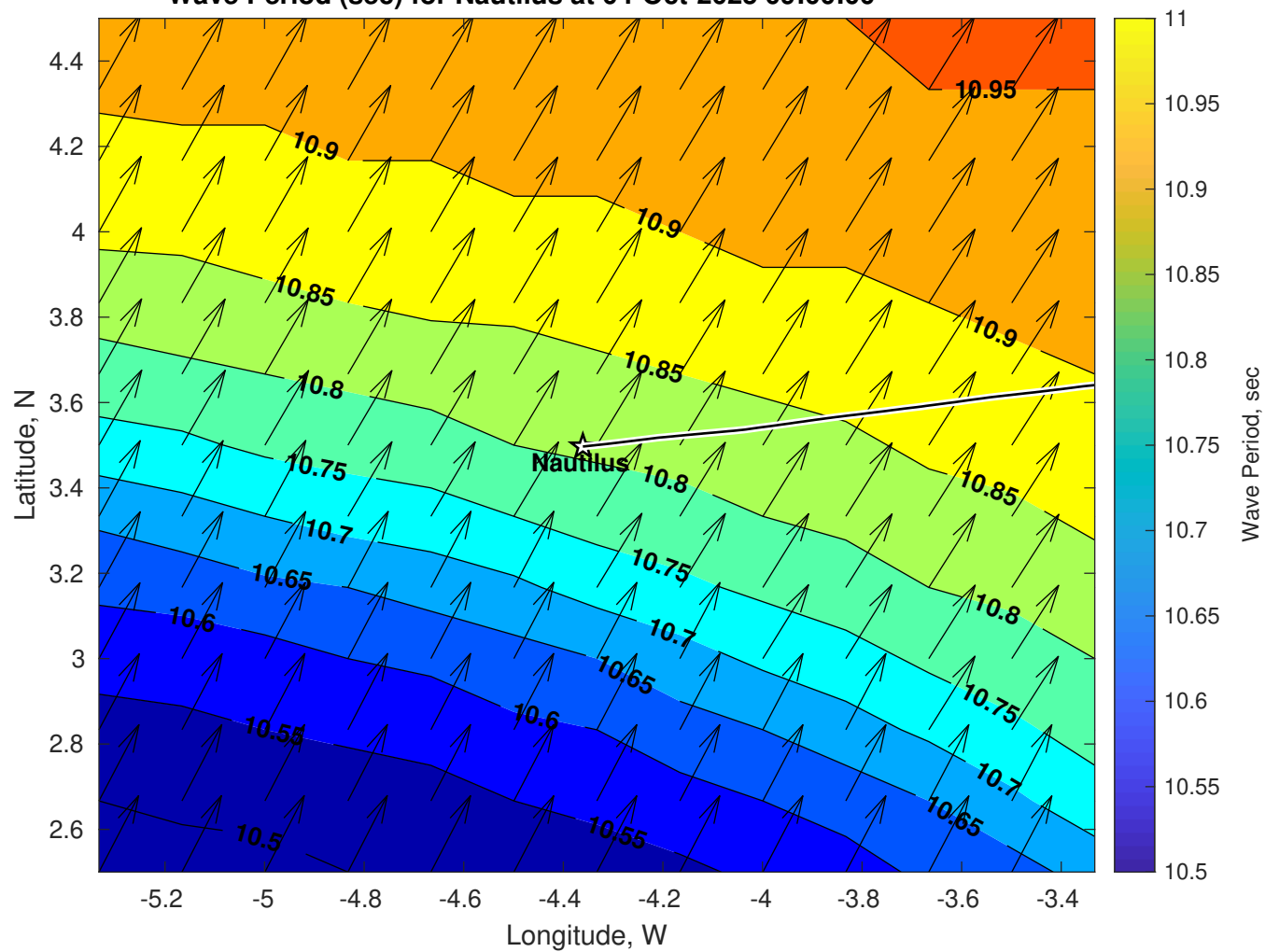
Wave Period (sec) for Nautilus at 04-Oct-2025 09:00:00
