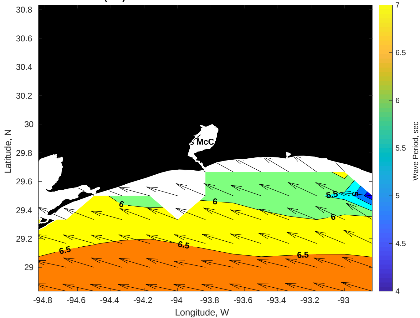
Wave Period (sec) for Brooks McCall at 05-Oct-2025 09:00:00
