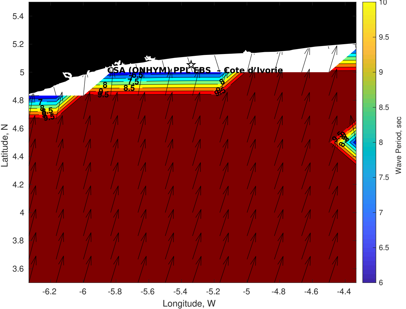
Wave Period (sec) for CSA (ONHYM) PPL EBS - Cote d'Ivoire at 05-Oct-2025 09:00:00
