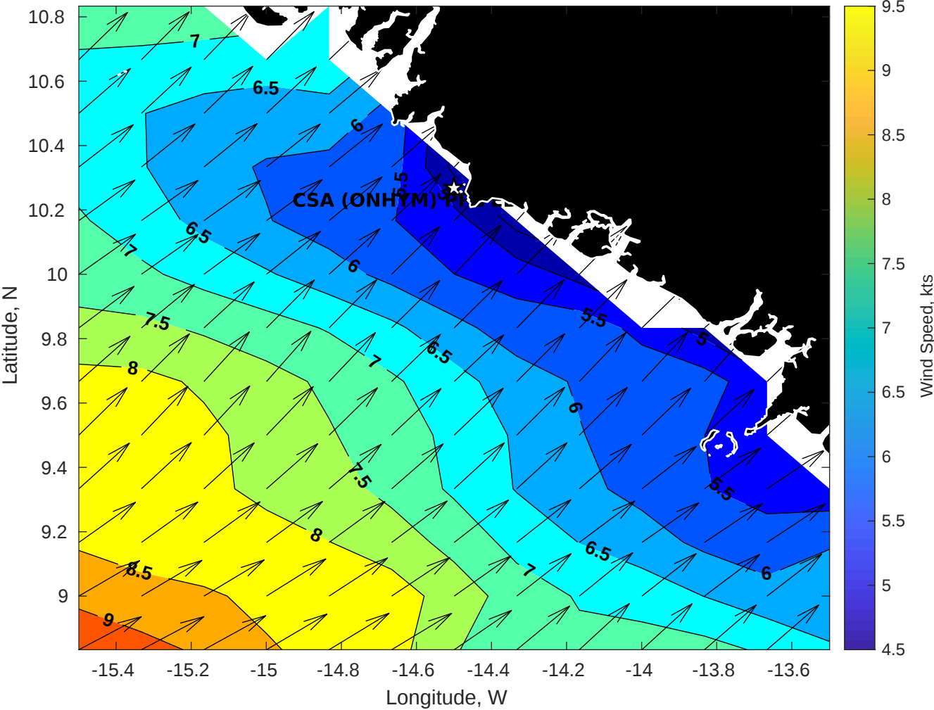
Winds (kts) for CSA (ONHYM) PPL EBS - Guinea at 05-Oct-2025 09:00:00
