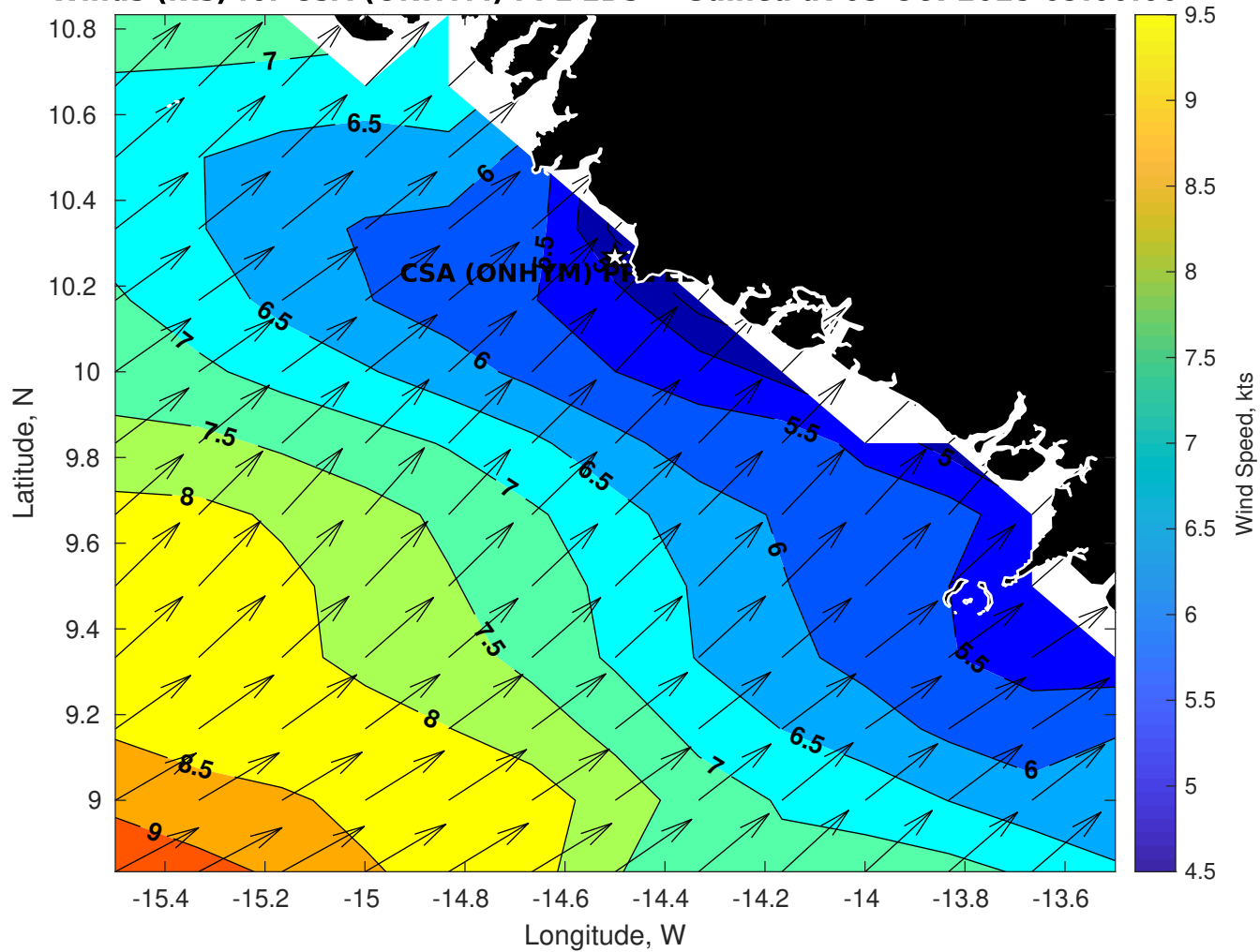
Winds (kts) for CSA (ONHYM) PPL EBS - Guinea at 05-Oct-2025 09:00:00
