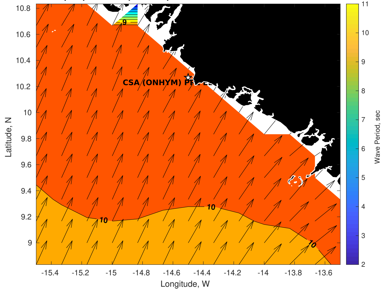
Wave Period (sec) for CSA (ONHYM) PPL EBS - Guinea at 05-Oct-2025 09:00:00
