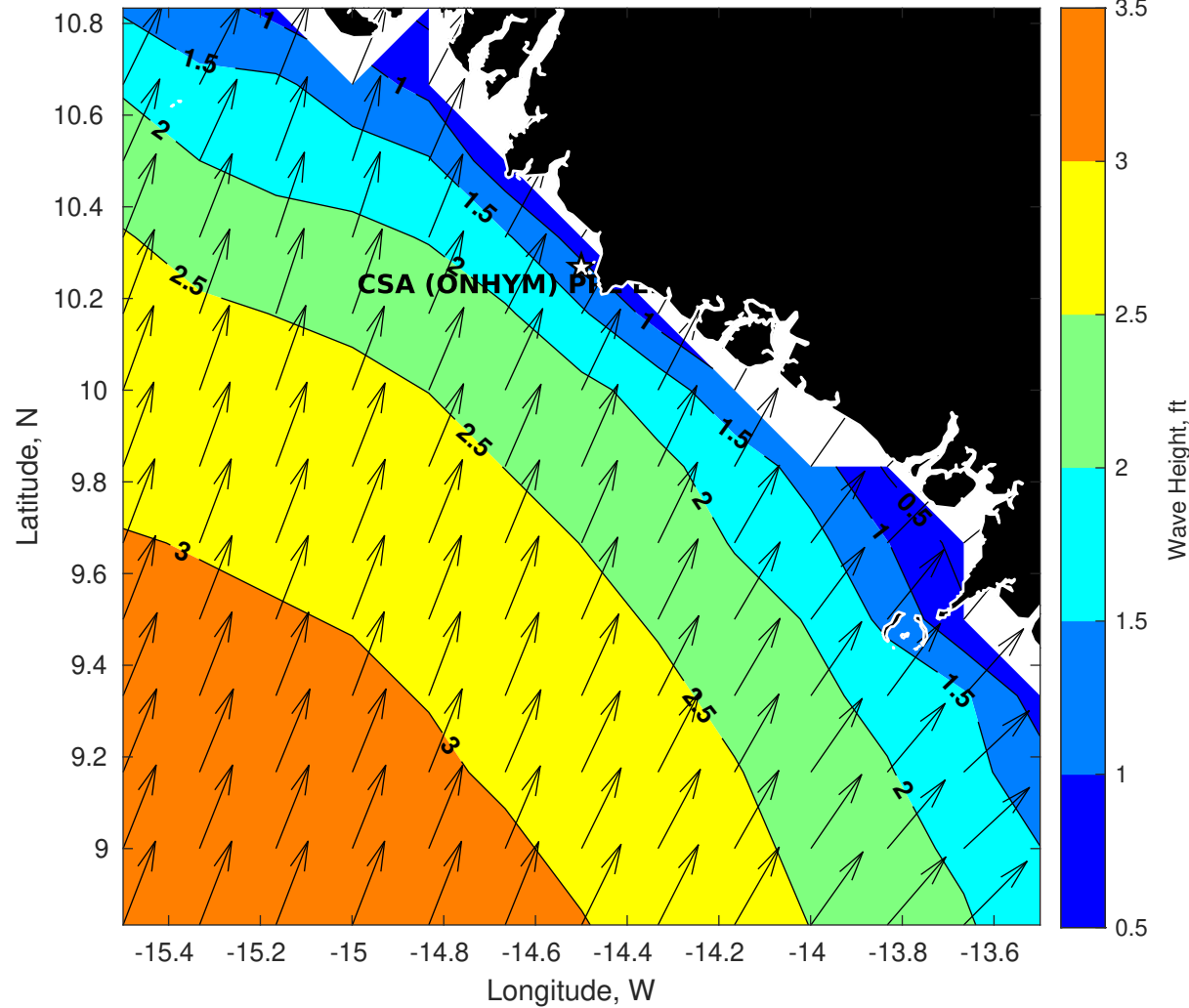
Wave Height (ft) for CSA (ONHYM) PPL EBS - Guinea at 05-Oct-2025 09:00:00
