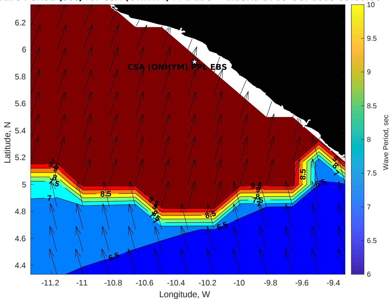
Wave Period (sec) for CSA (ONHYM) PPL EBS - Liberia at 05-Oct-2025 09:00:00
