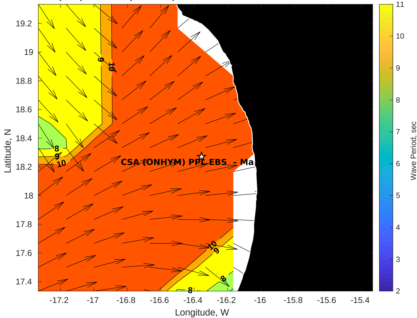
Wave Period (sec) for CSA (ONHYM) PPL EBS - Mauritania at 05-Oct-2025 09:00:00
