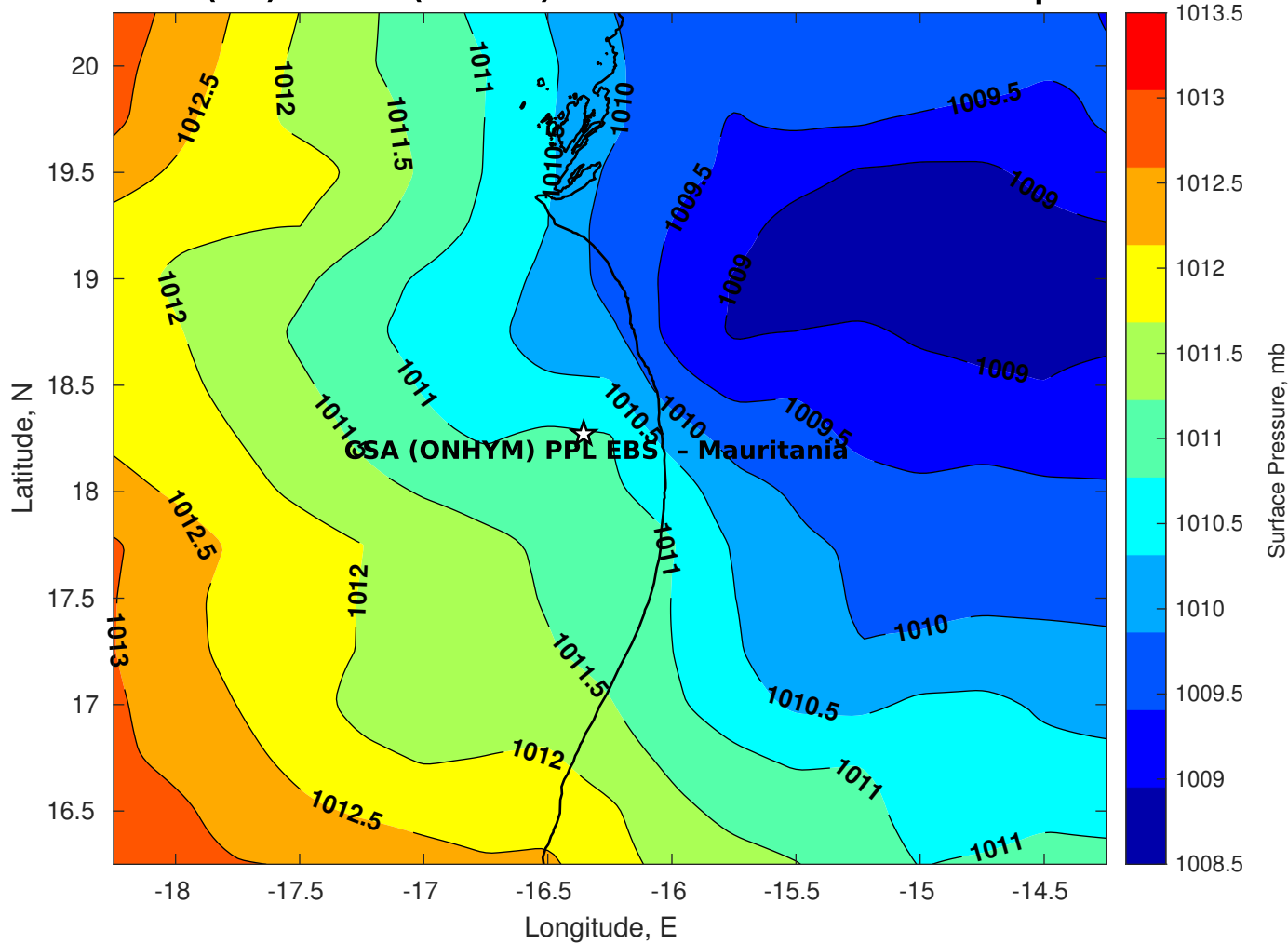
Surface Pressure (mb) for CSA (ONHYM) PPL EBS - Mauritania at 18-Sep-2025 12:00:00
