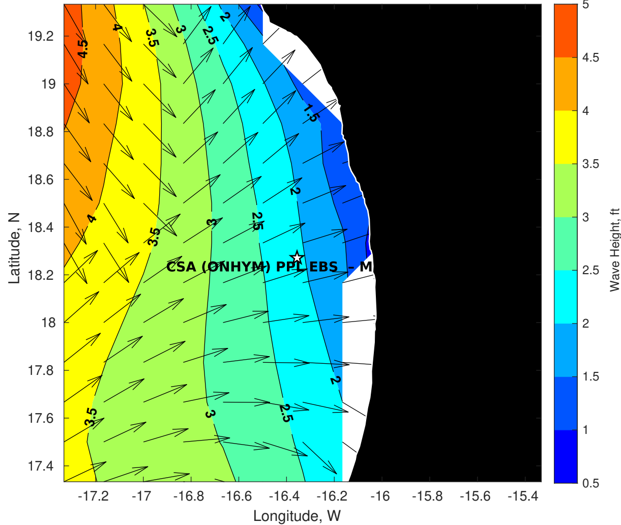
Wave Height (ft) for CSA (ONHYM) PPL EBS - Mauritania at 05-Oct-2025 09:00:00
