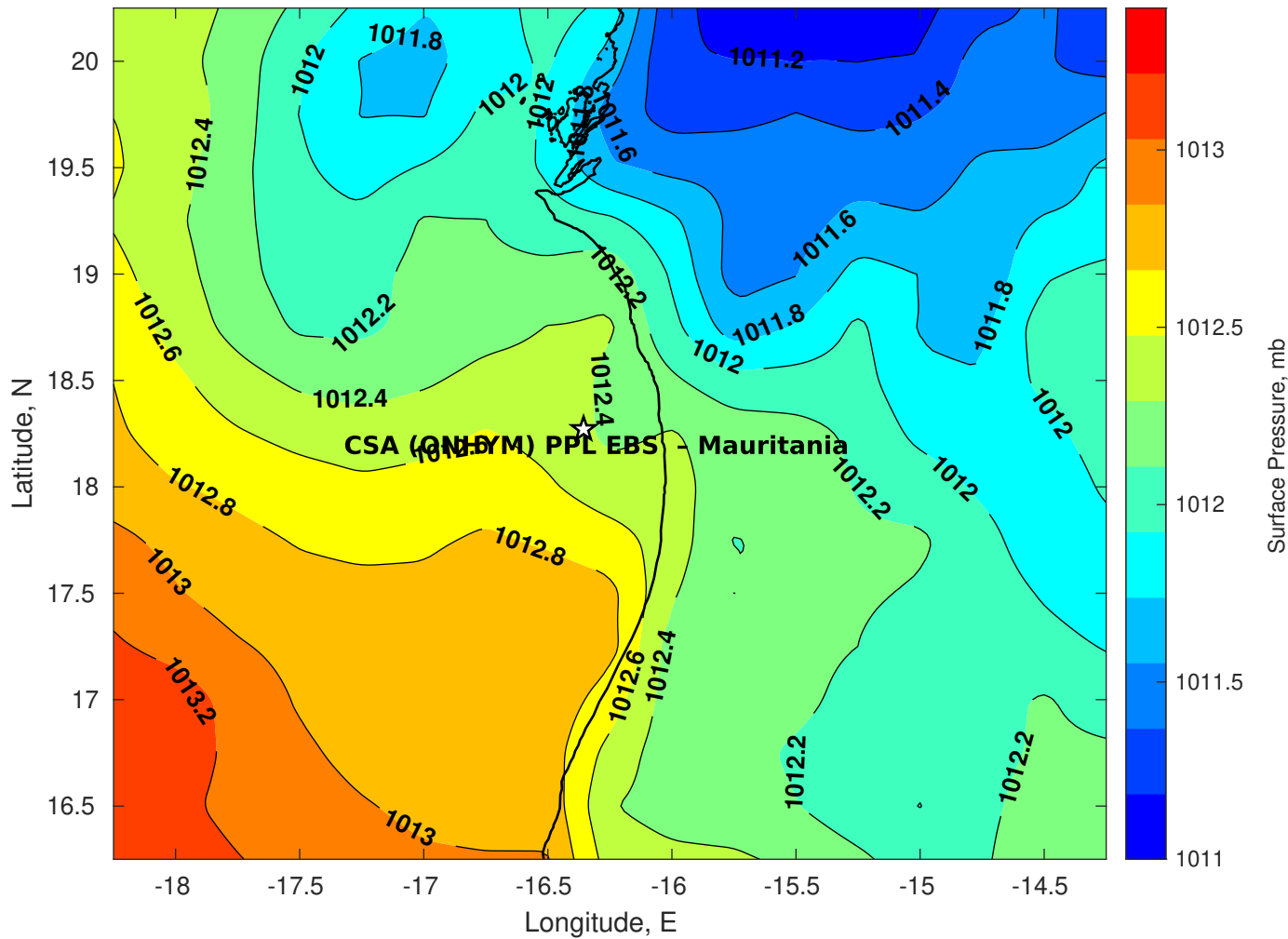
Surface Pressure (mb) for CSA (ONHYM) PPL EBS - Mauritania at 19-Sep-2025 12:00:00
