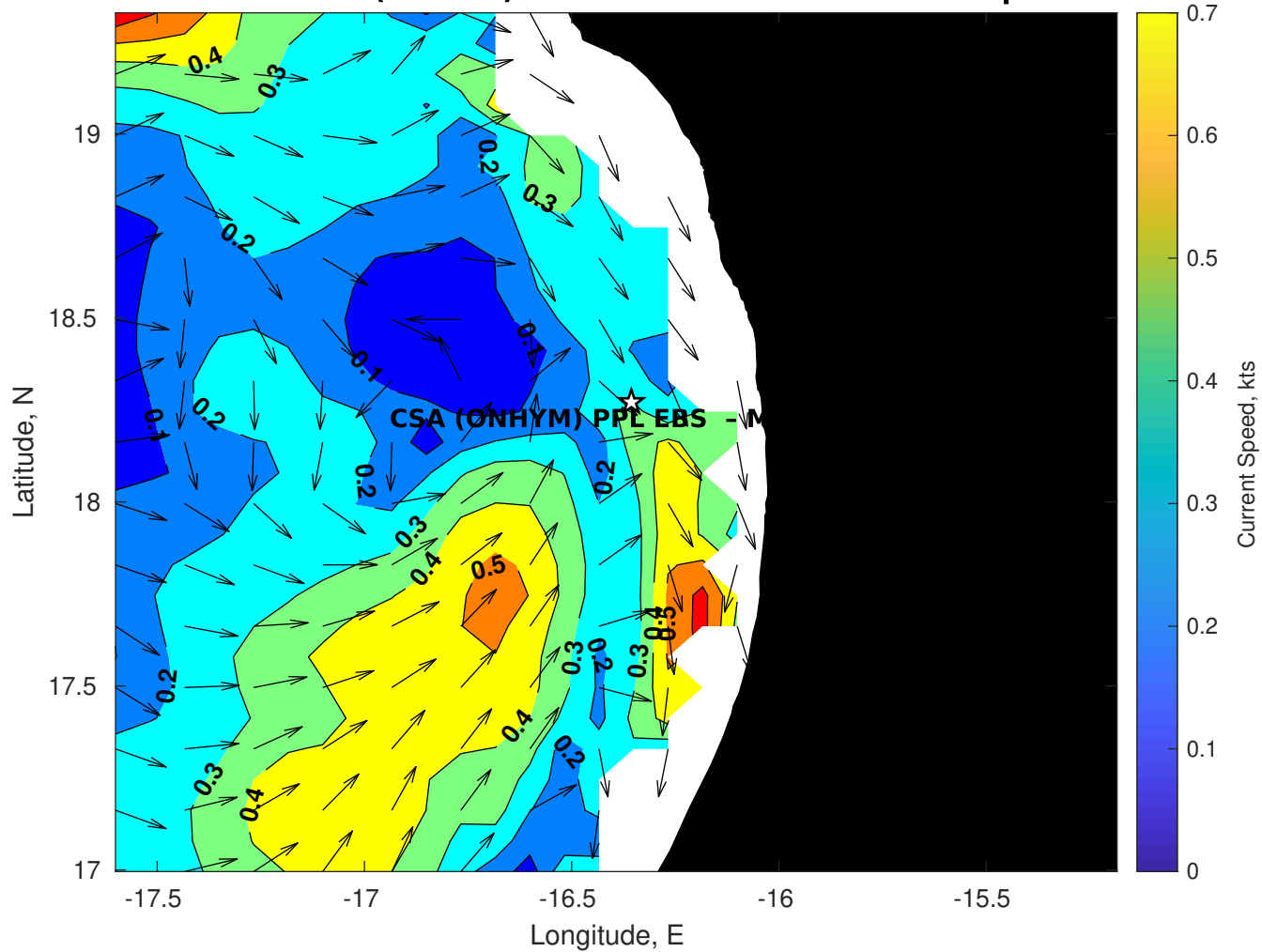
Surface Currents for CSA (ONHYM) PPL EBS - Mauritania at 17-Sep-2025 00:00:00
