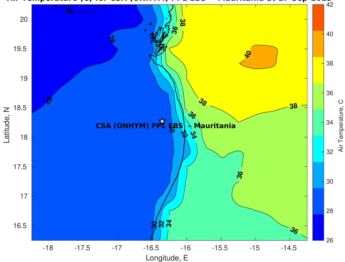
Air Temperature (C) for CSA (ONHYM) PPL EBS - Mauritania at 17-Sep-2025
