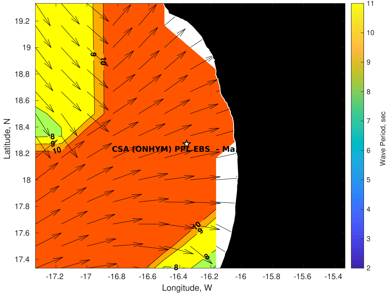
Wave Period (sec) for CSA (ONHYM) PPL EBS - Mauritania at 05-Oct-2025 09:00:00
