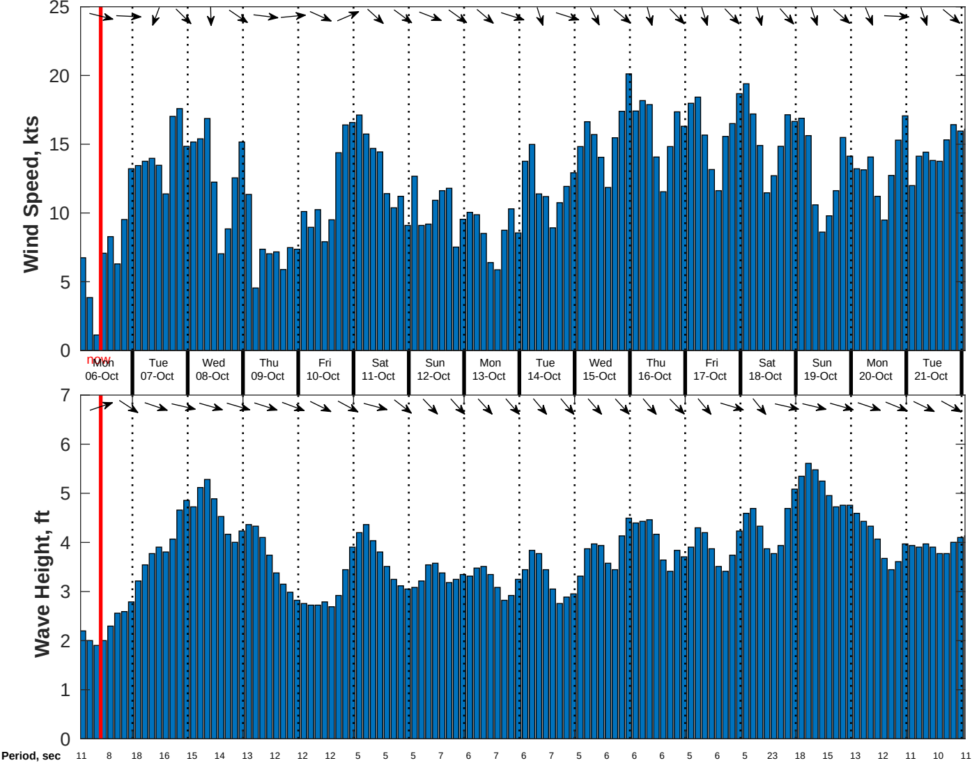
Wind & Wave Forecast for CSA (ONHYM) PPL EBS - Mauritania from 05-Oct-2025 01:00:00 to 21-Oct-2025 01:00:00
