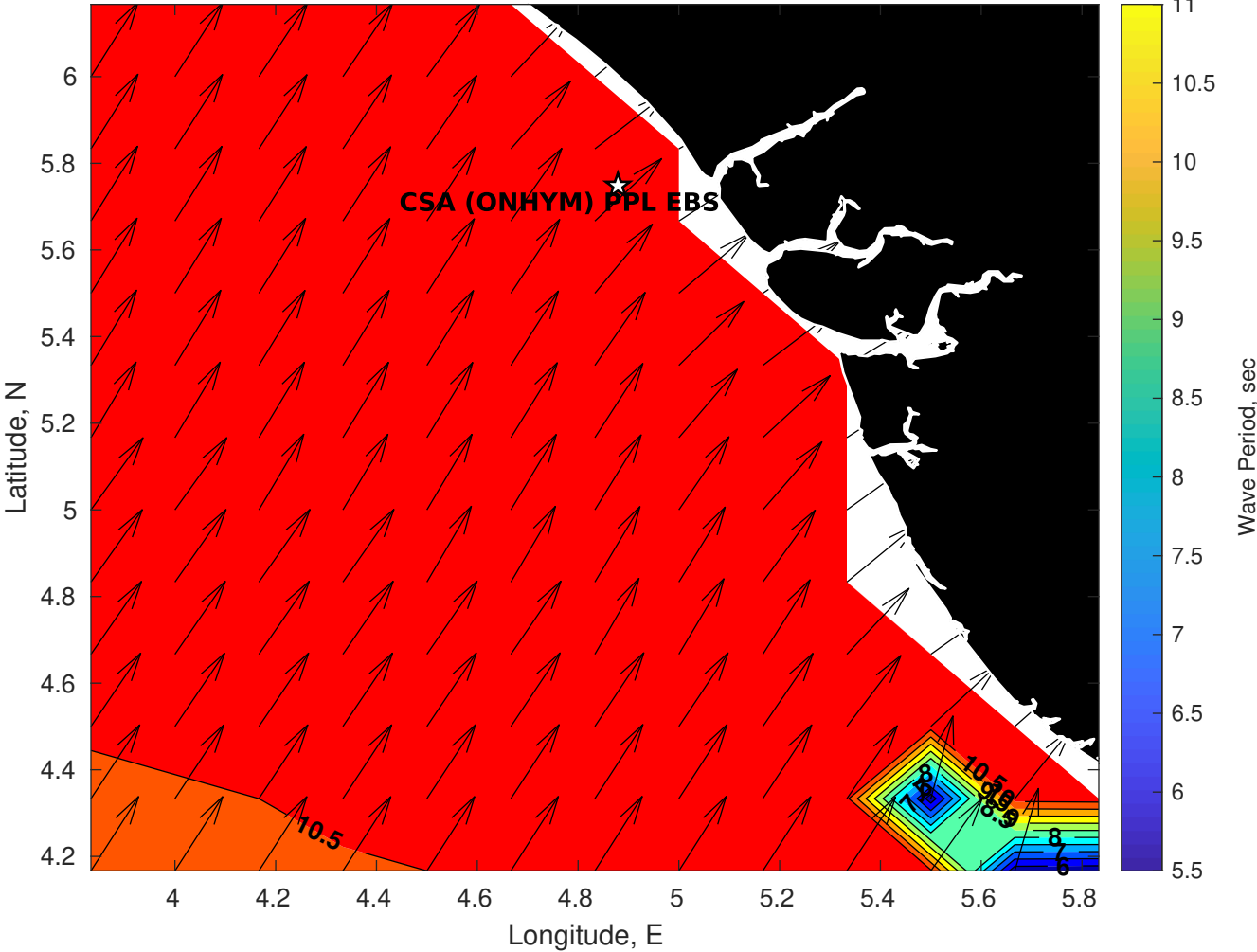
Wave Period (sec) for CSA (ONHYM) PPL EBS - Nigeria at 05-Oct-2025 09:00:00
