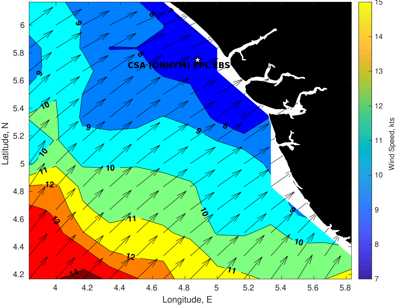
Winds (kts) for CSA (ONHYM) PPL EBS - Nigeria at 05-Oct-2025 09:00:00
