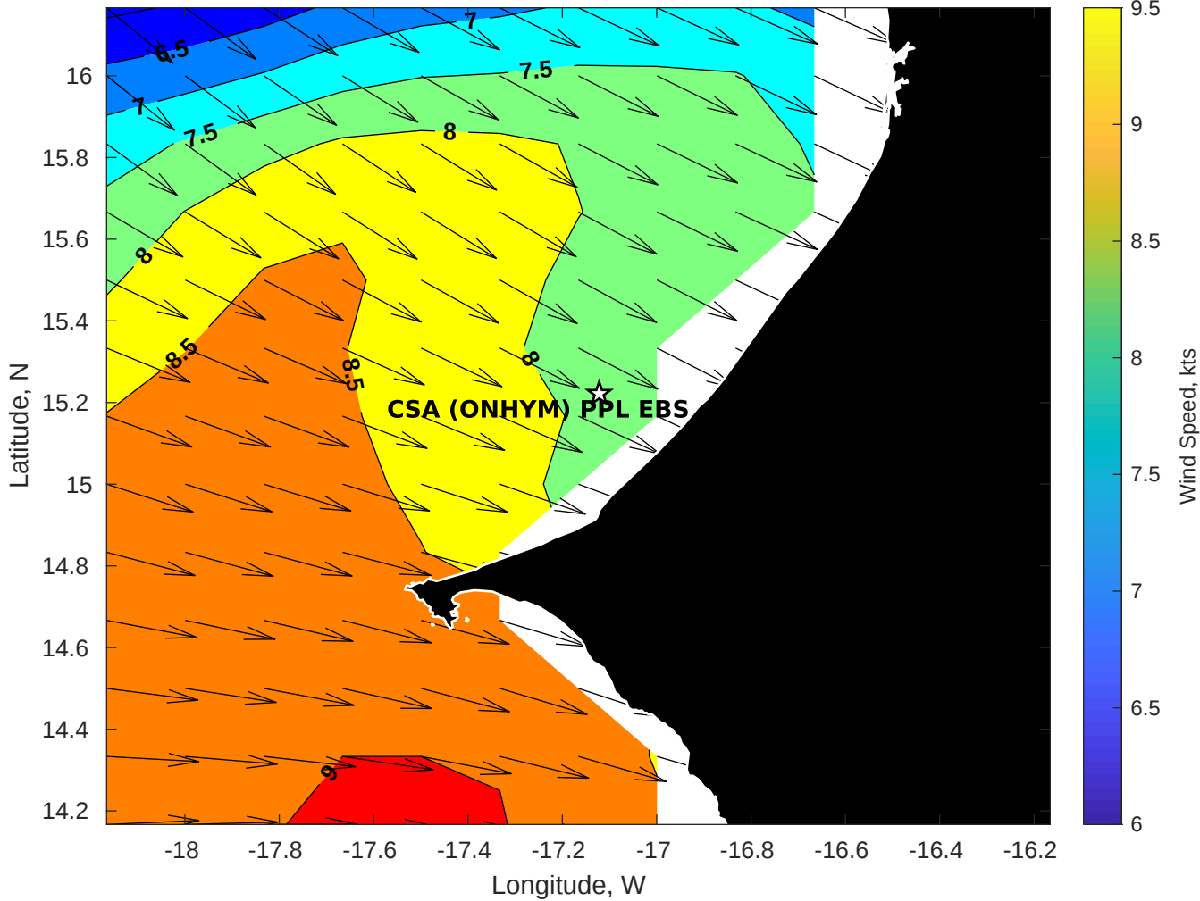
Winds (kts) for CSA (ONHYM) PPL EBS - Senegal at 05-Oct-2025 09:00:00
