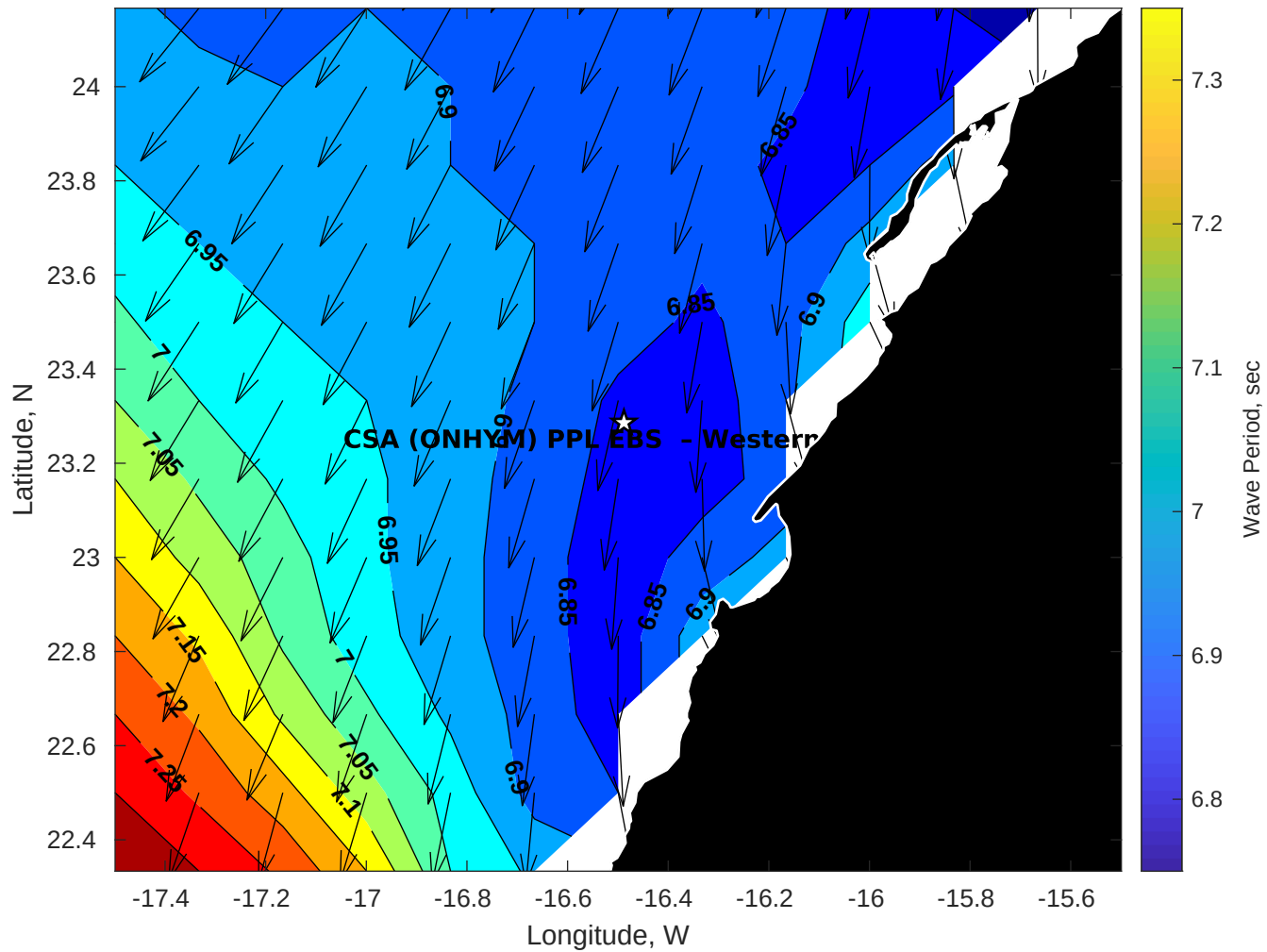
Wave Period (sec) for CSA (ONHYM) PPL EBS - Western Sahara at 05-Oct-2025 09:00:00
