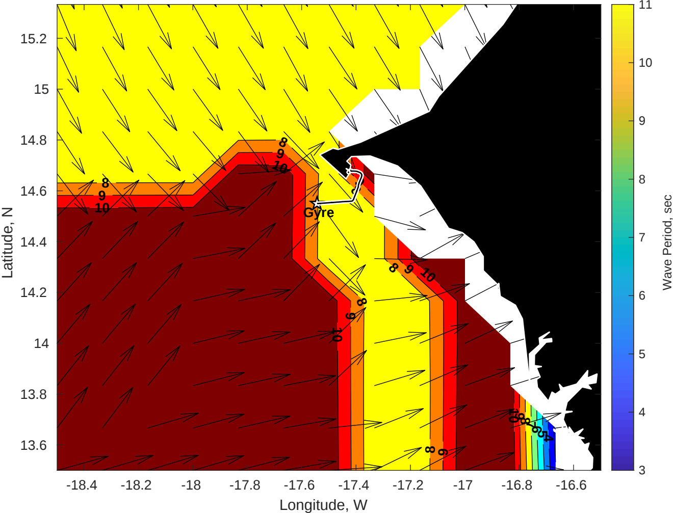
Wave Period (sec) for Gyre at 05-Oct-2025 09:00:00
