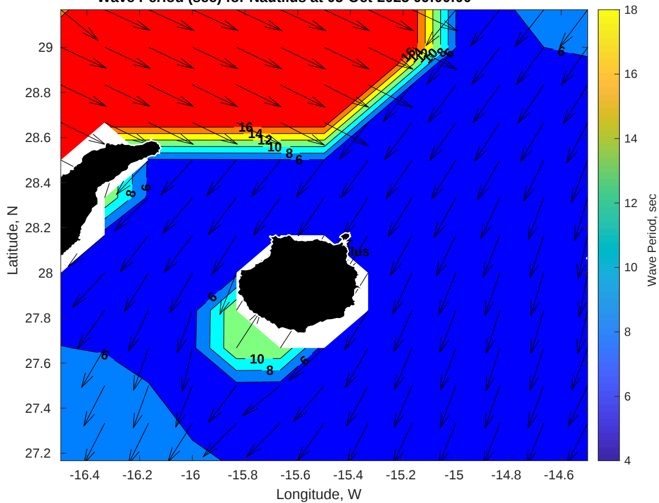
Wave Period (sec) for Nautilus at 05-Oct-2025 09:00:00
