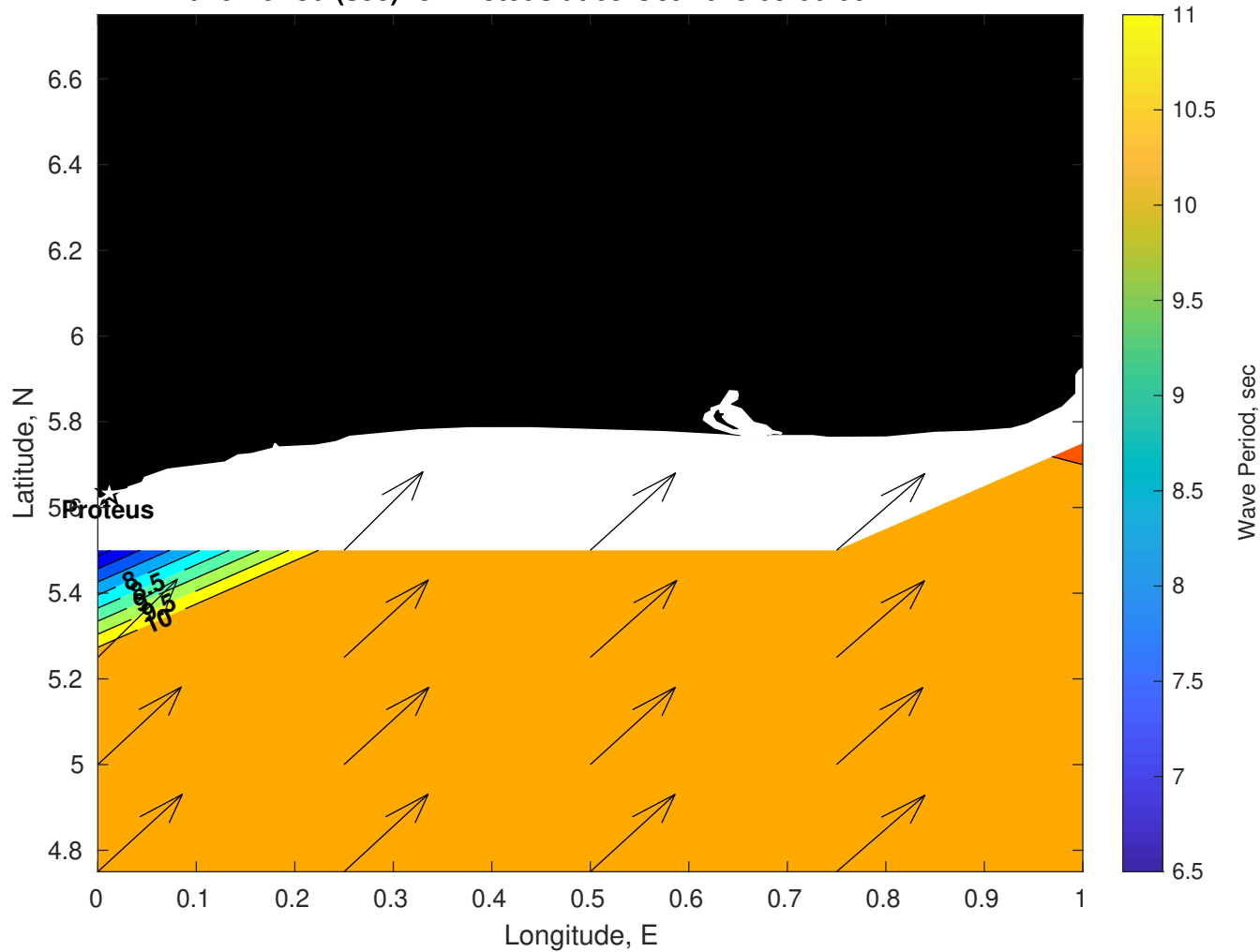
Wave Period (sec) for Proteus at 05-Oct-2025 09:00:00
