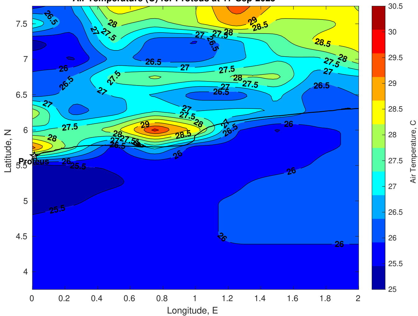
Air Temperature (C) for Proteus at 17-Sep-2025
