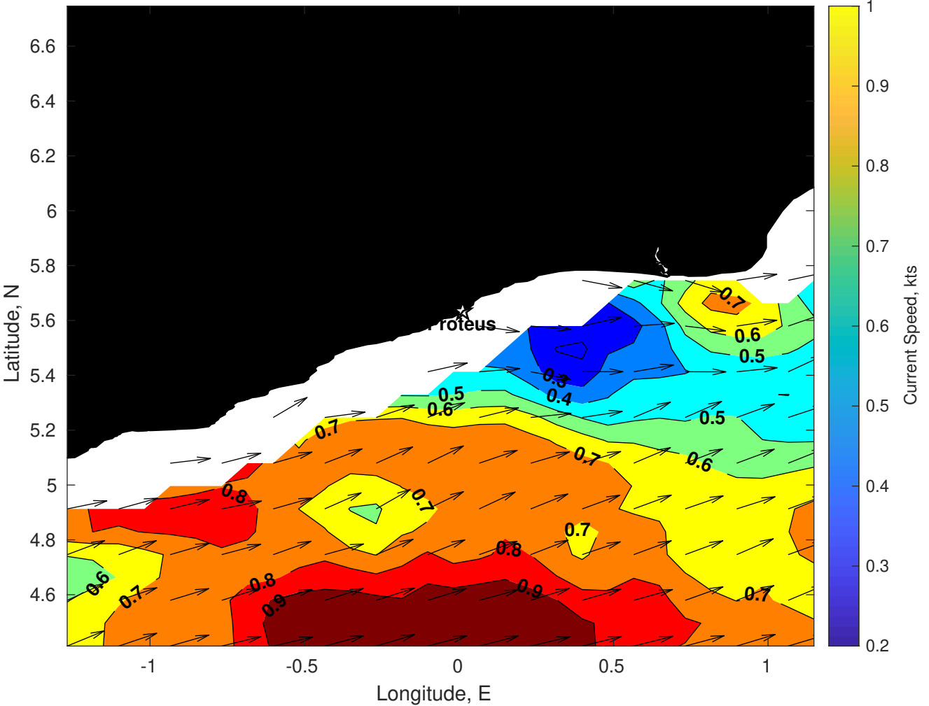
Surface Currents for Proteus at 17-Sep-2025 00:00:00
