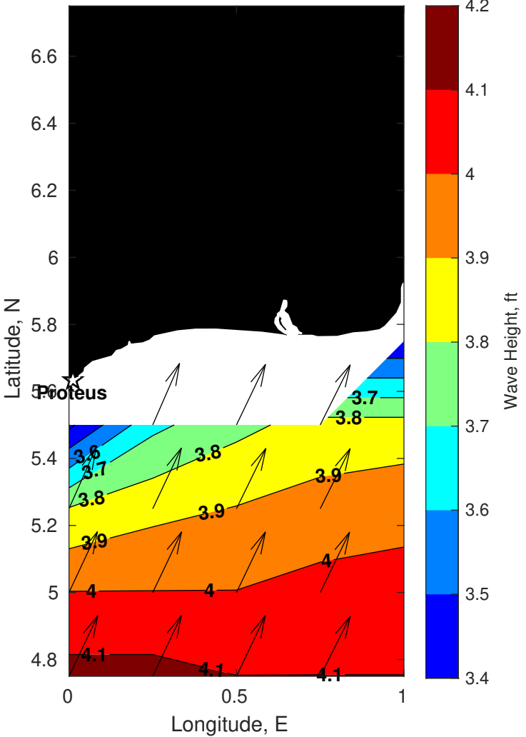
Wave Height (ft) for Proteus at 05-Oct-2025 09:00:00
