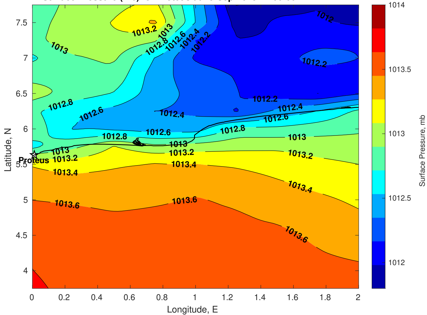
Surface Pressure (mb) for Proteus at 18-Sep-2025 12:00:00
