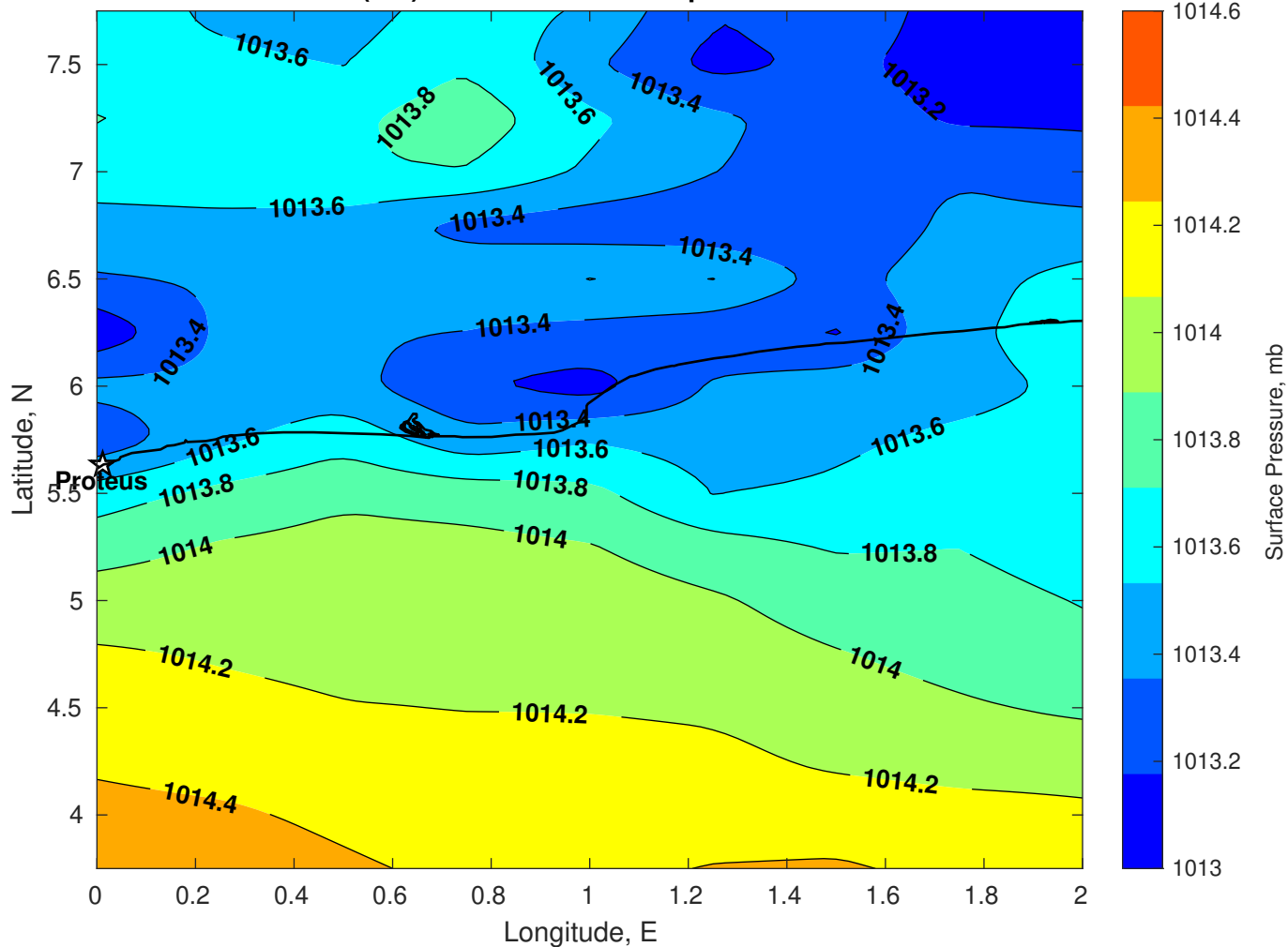
Surface Pressure (mb) for Proteus at 19-Sep-2025 12:00:00
