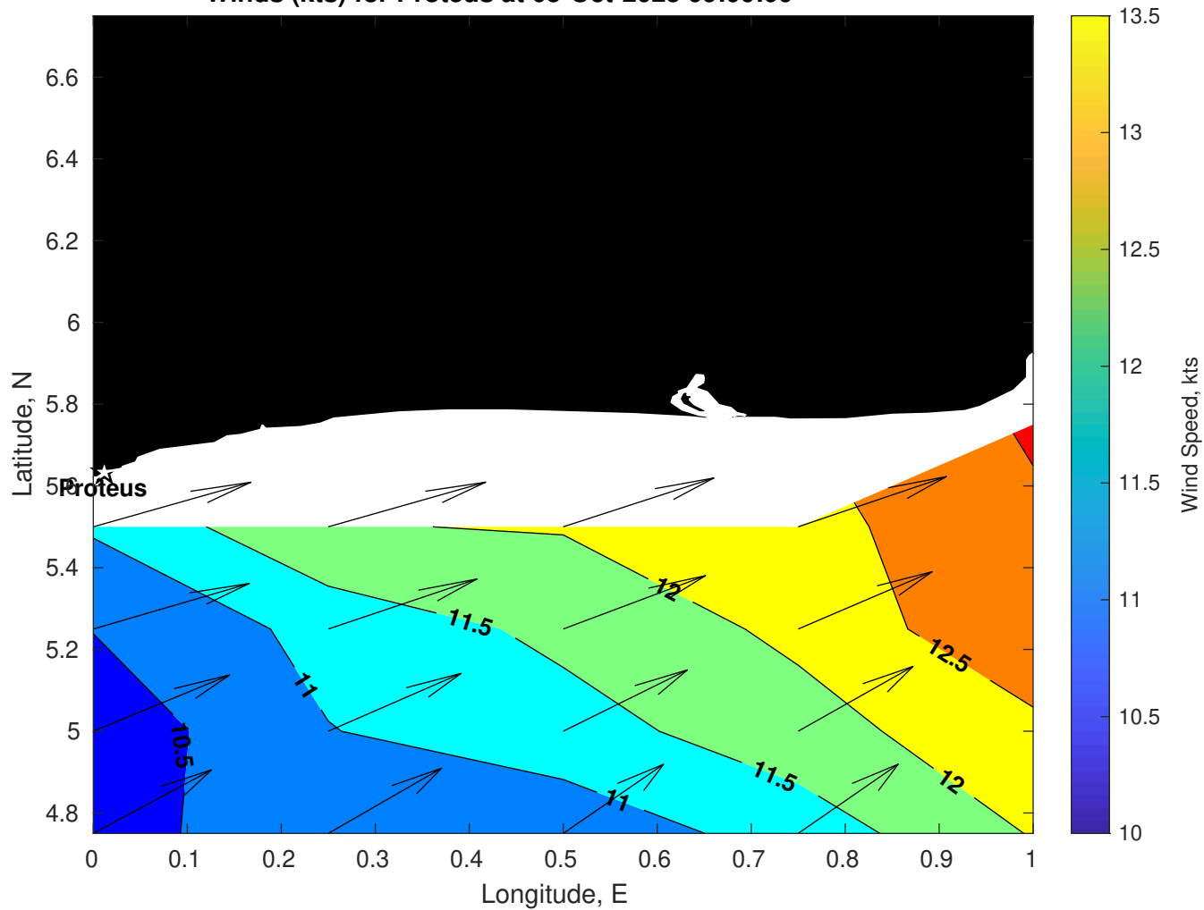
Winds (kts) for Proteus at 05-Oct-2025 09:00:00
